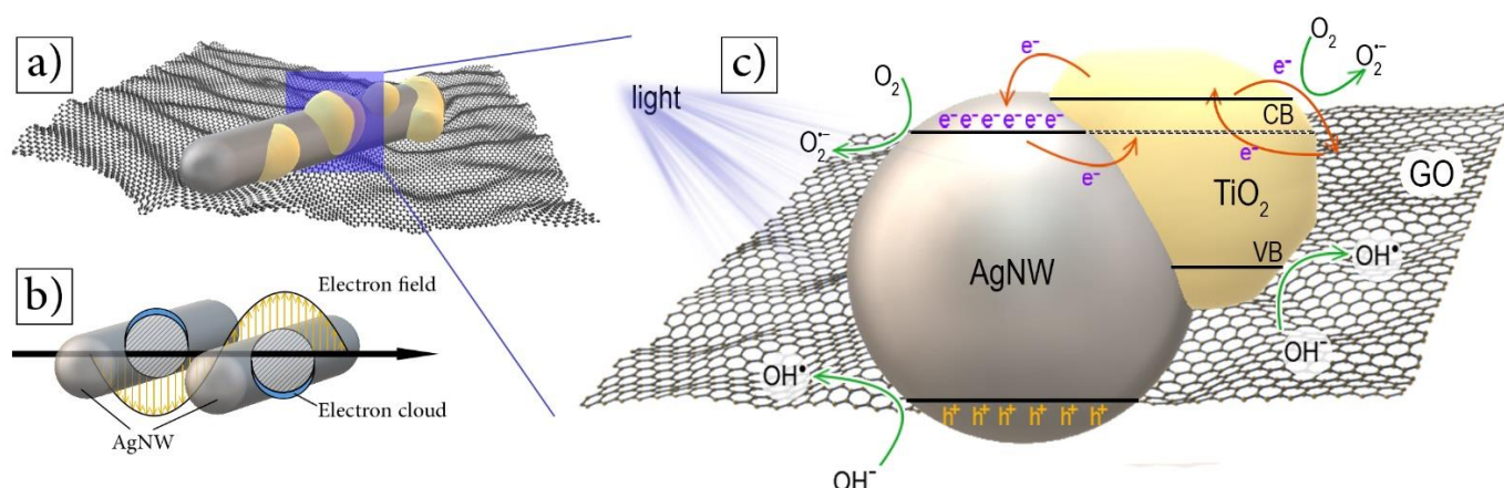
Figure 11. Schematic diagrams of (a) AgNW/TiO 2 /GO nanocomposite structure, (b) localized SPR of AgNWs when irradiated with visible or UV light, and (c) photocatalytic mechanism of AgNW/TiO 2 /GO nanocomposites.
