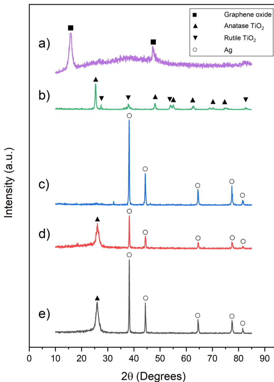
Figure 3. X-ray diffraction patterns of (a) GO, (b) P25 TiO 2 , (c) AgNW (d) AgNW/TiO 2 , and (e) AgNW/TiO 2 /GO samples.
