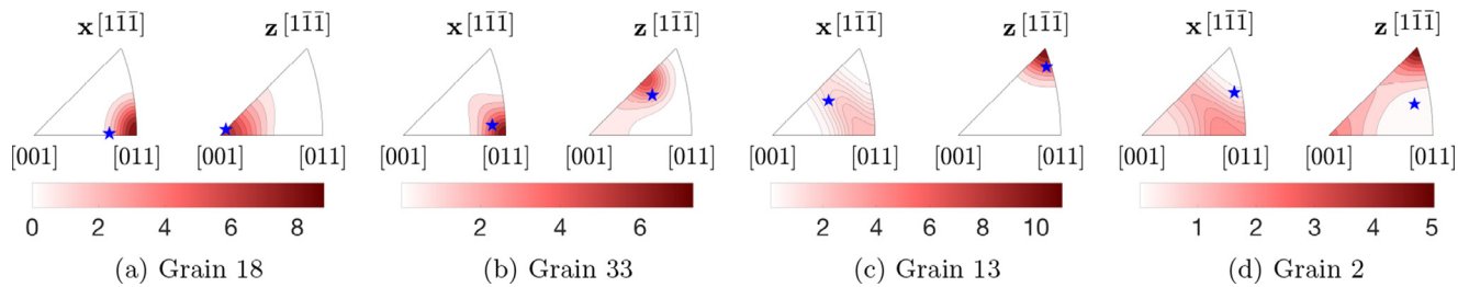
Fig. 6. Inverse pole figure distribution map with respect to the loading direction (z) and stretching direction (x) for four selected grains. (a) A Grain close to the rotated cube orientation with minimal deformation heterogeneity; (b) A grain belonging to the \alpha -fiber showing a small tendency to form in-grain misorientation spread; (c) A grain belonging to the \gamma -fiber showing a strong tendency to form in-grain misorientation spread compared to the \alpha -fiber; (d) A grain fragmented into regions of distinctly different orientations. The grains are defined based on the initial microstructure before deformation (see Fig. 5b), and the blue stars show the initial orientations. (For interpretation of the references to colour in this figure legend, the reader is referred to the web version of this article.)
