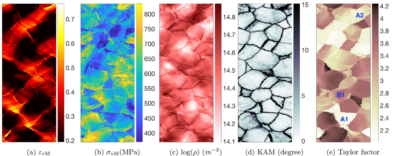
Fig. 9. Simulation results at the mid-surface after a 20% thickness reduction; (a) equivalent strain \varepsilon_{vM} , (b) equivalent stress \sigma_{vM} (MPa), (c) \log(\rho) ( m^{-2} ), (d) KAM (degree), (e) Taylor factor with respect to the loading (vertical) direction.
