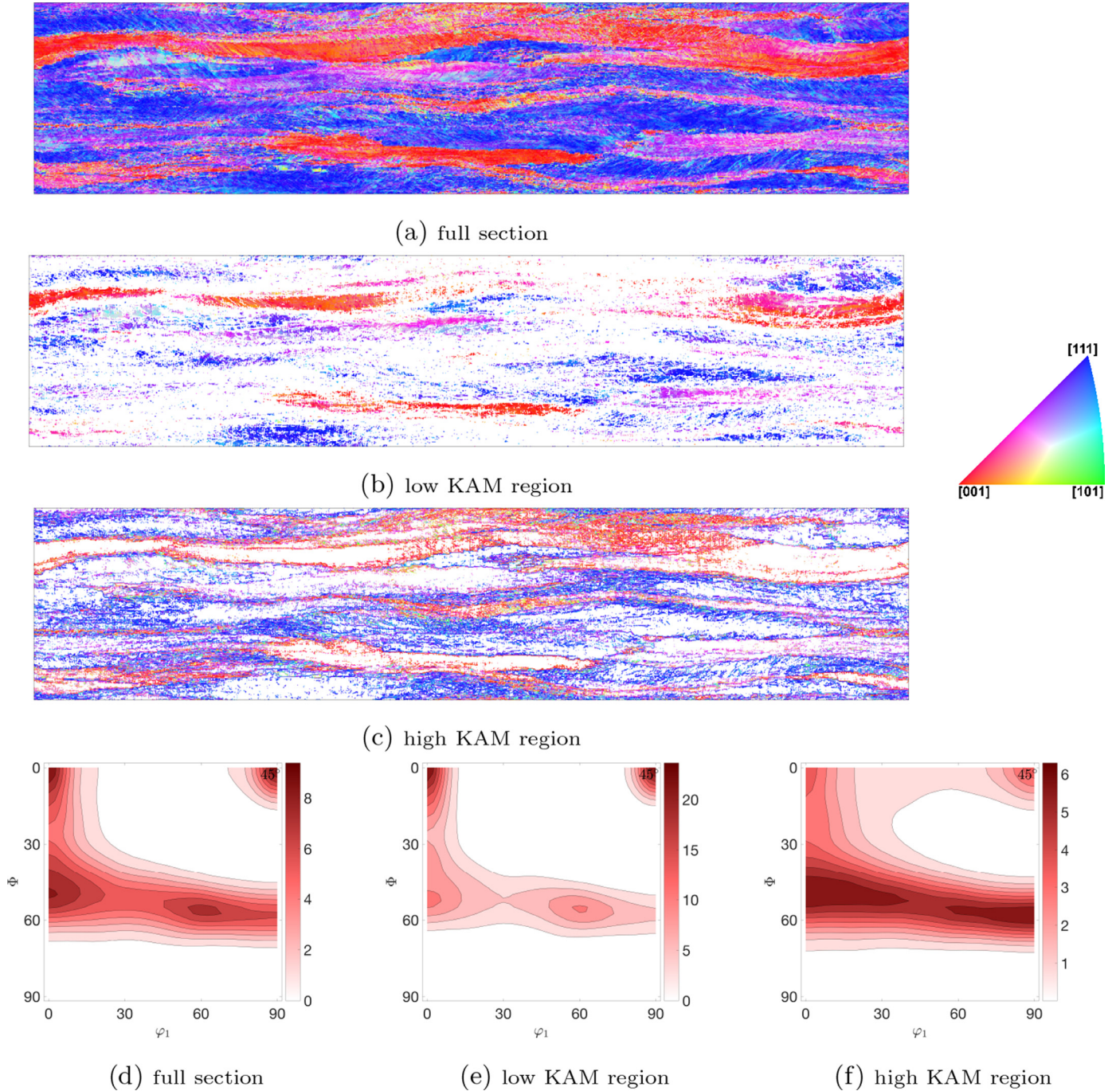
Fig. 2. Simulation results showing the low and high KAM regions in the mid-surface of the 3D simulation after 77% thickness reduction. (a–c) IPF color maps parallel to the loading (vertical) direction, (d–f) orientation density f(g) maps obtained from the ODF section \phi_2 = 45^\circ .
