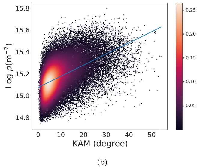
Fig. 19. (a) Correlation between the dislocation density and main variables. (b) 2D probability density plot of the dislocation density and KAM. The blue line shows the linear regression line. (For interpretation of the references to colour in this figure legend, the reader is referred to the web version of this article.)
