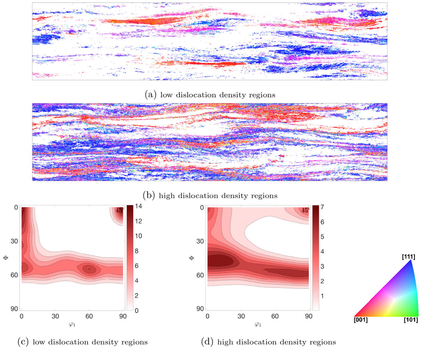
Fig. 17. Simulation results showing low and high dislocation density regions. (a,b) IPF color maps parallel to the loading (vertical) direction, (c,d) orientation density f(\phi) maps obtained from the ODF section \phi_2 = 45^\circ .
