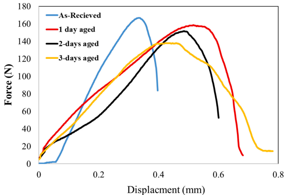
Fig. 5. Shear force vs. displacement of different ageing time at 150 °C.
