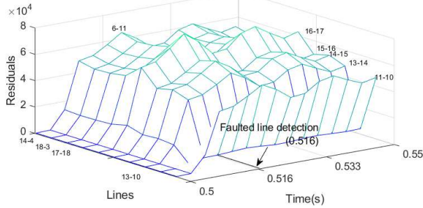
Figure 10. Residuals used to localize the faulted line
