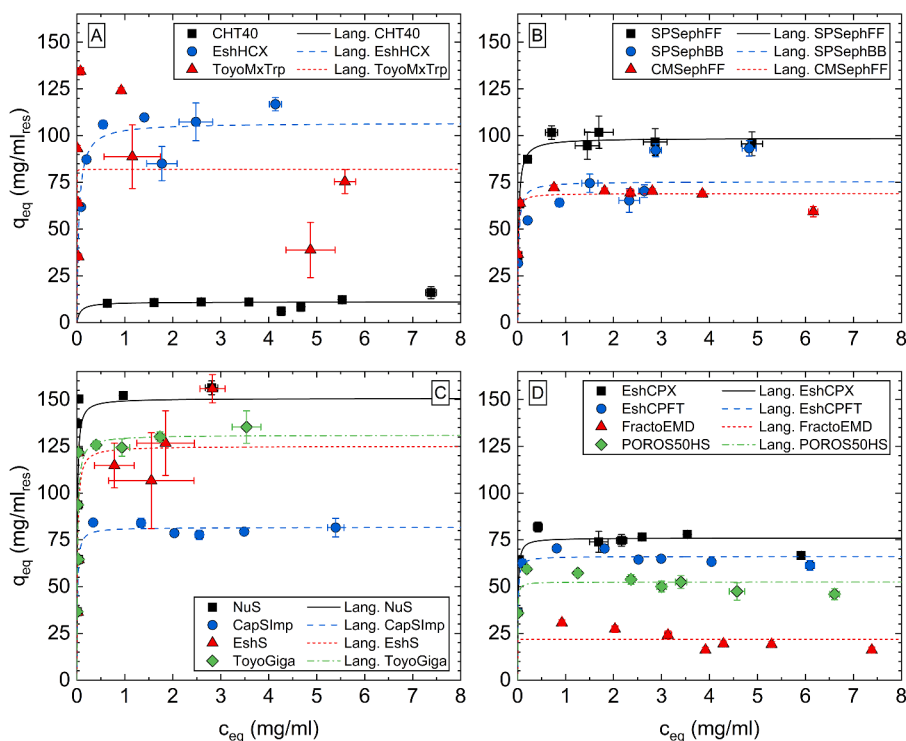
Fig. 3. Adsorption isotherms of mAb on different CEX resins in 25 mM NaOAc buffer, pH 4.5. A – Multimodal CEX resins; B – Sepharose resins; C – -SO_3^- functional group resins; D – Sulfoisobutyl (Eshmuno CPX and CPFT and Fractogel EMD COO^- ) and sulfopropyl (POROS 50 HS) functional group resins).
