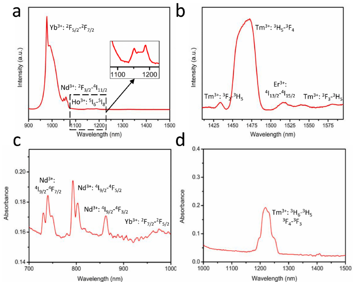
Fig. 3. (a) Room temperature luminescence emission spectrum of \text{NaYF}_4:\text{Yb}^{3+}, \text{Ho}^{3+}@\text{NaYF}_4:\text{Nd}^{3+}/\text{SiO}_2 aqueous suspension under excitation at 808 nm. (b) Room temperature luminescence emission spectrum of \text{NaYF}_4:\text{Tm}^{3+}, \text{Er}^{3+}@\text{NaYF}_4/\text{SiO}_2 aqueous suspension under excitation at 1208 nm. Absorption spectra of (c) \text{NaYF}_4:\text{Yb}^{3+}, \text{Ho}^{3+}@\text{NaYF}_4:\text{Nd}^{3+}/\text{SiO}_2 and (d) \text{NaYF}_4:\text{Tm}^{3+}, \text{Er}^{3+}@\text{NaYF}_4/\text{SiO}_2 .
