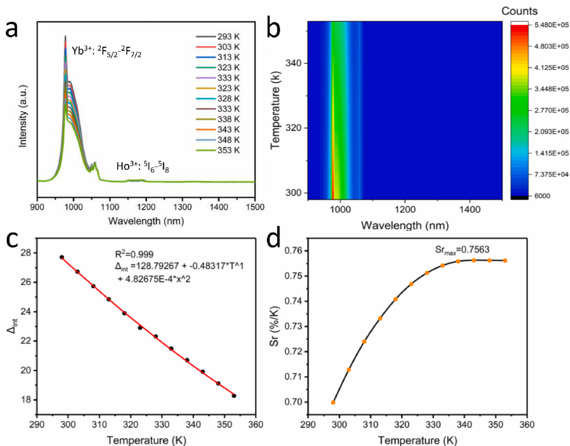
Fig. 5. (a, b) Temperature-dependent NIR emission spectra of NaYF 4 :Yb 3+ , Ho 3+ @NaYF 4 :Nd 3+ @SiO 2 aqueous suspension under 808 nm excitation. (c) Calibration curve for the relationship between \Delta_{int} and temperature of the NaYF 4 :Yb 3+ , Ho 3+ @NaYF 4 :Nd 3+ @SiO 2 aqueous suspension. (d) S_r values at different temperatures for the NaYF 4 :Yb 3+ , Ho 3+ @NaYF 4 :Nd 3+ @SiO 2 aqueous suspension.
