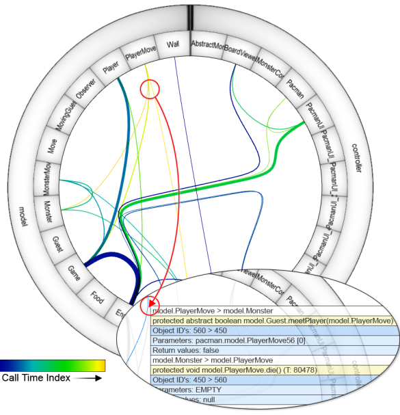
Figure 6. Circular, temporal view of the “player dies” feature that shows runtime information.
