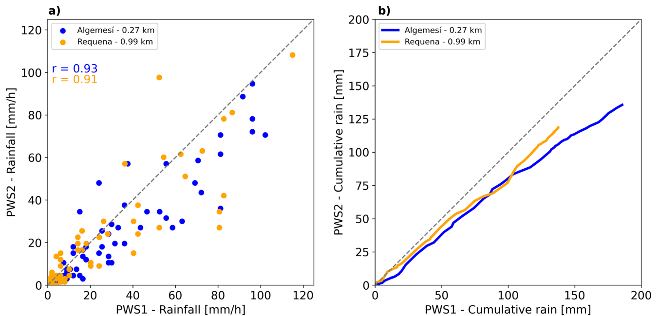
Figure 4. (a) Scatter plot of 5 min rainfall between two pairs of PWSs (in Requena and Algemesí, indicated with B and E in Fig. 1c), with an inter-gauge distance of less than 1 km. The correlation coefficient ( r ) quantifies the relation between the stations. (b) Cumulative rainfall between two pairs. Only intervals where both stations contain measurements are included. Legend indicates in which town the PWSs were located and the inter-gauge distance.
