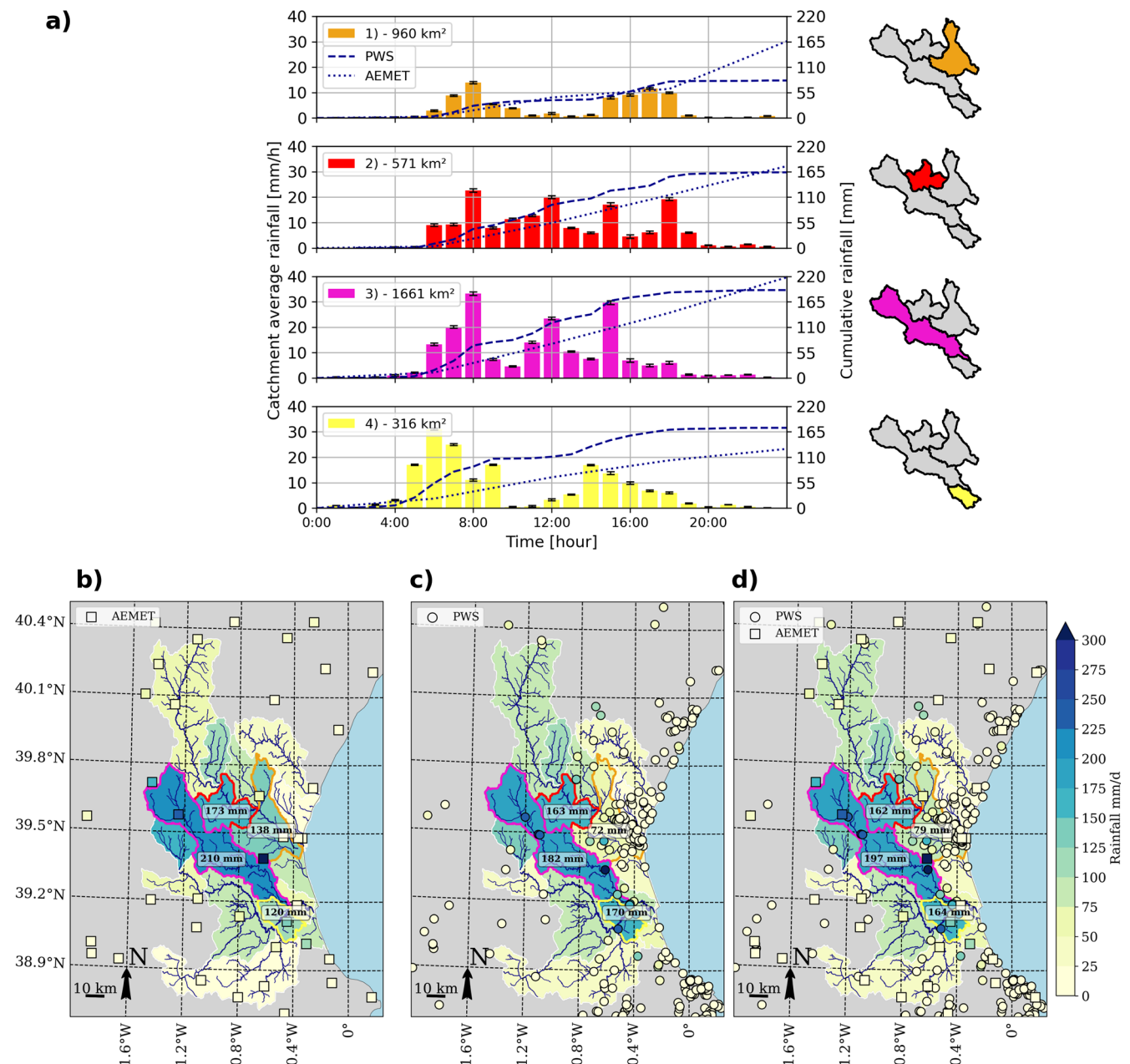
Figure 6. (a) Catchment-average rainfall over time (local time) based on PWS data for four catchments that were affected by torrential rainfall and/or severely flooded, with the error bar indicating the uncertainty associated with kriging. Dashed line is the cumulative rainfall based on the hourly PWS data, dotted line is based on the 6 h AEMET data. Lower panel shows the catchment-average rainfall over the whole day based on (b) AEMET stations (c) PWSs and (d) AEMET and PWSs combined. The numbers in the catchments indicate the average accumulated rain. Colours in (1)–(4) in (a) correspond with the catchments indicated with the same colour in (b–d).
