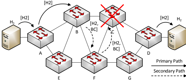
(a) Node failure at node C incorrectly handled by link-disjoint backup path
