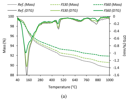
Fig. 10. TG-DTG (a) and DSC (b) curves of UHPC mixtures that were cured for 90 days.
