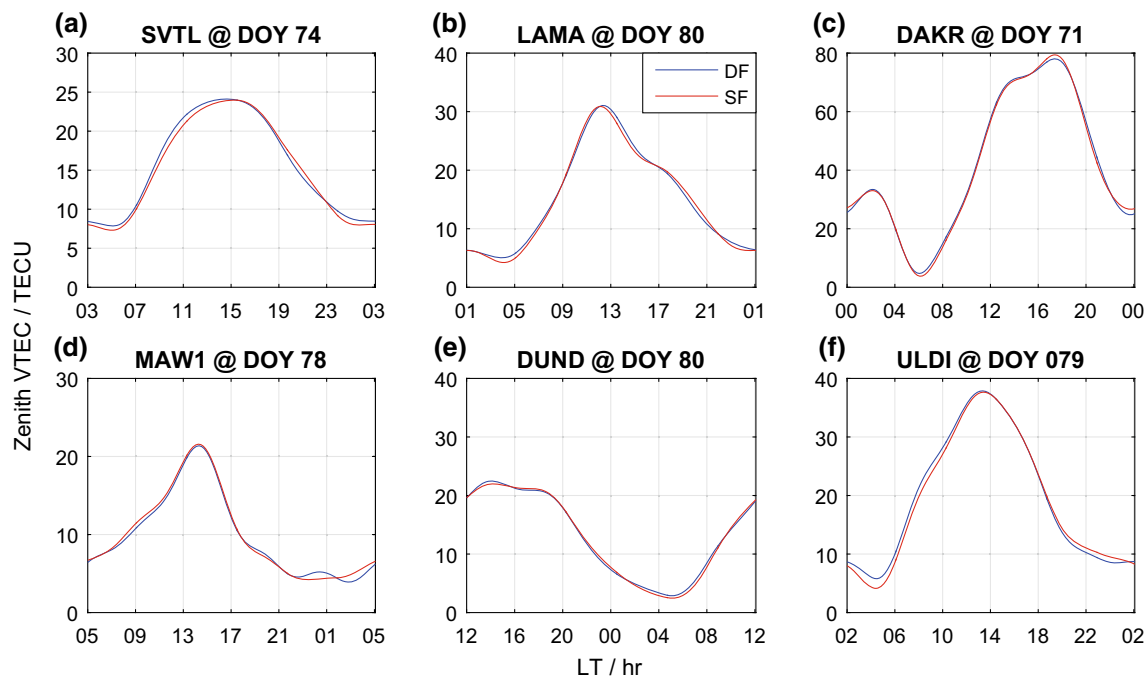
Fig. 7 a–f Analogous to those in Fig. 6, except that they show results for another six receivers spread throughout the globe and for a few days in March 2015
