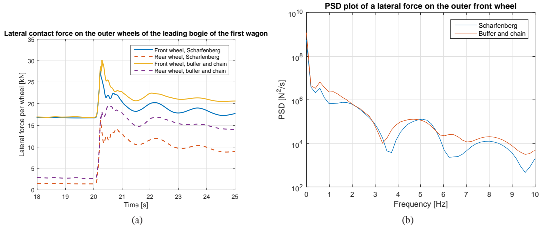
Figure 6 The lateral force on the outer wheels of the leading bogie of the first wagon in curve at 40 km/h. The vehicle is dynamically simulated steadily curving in a 260 m radius curve. At time 20 s the locomotive starts braking with a braking coefficient of 0.4.
