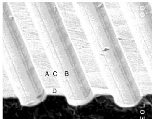
Figure 4. SEM image side view of a PVM periodical structure surface: A - photoactive mesa structure – photovoltaic cell, B - trench, C - non-metalized wall, D - non-metalized region of the device [13][14].
