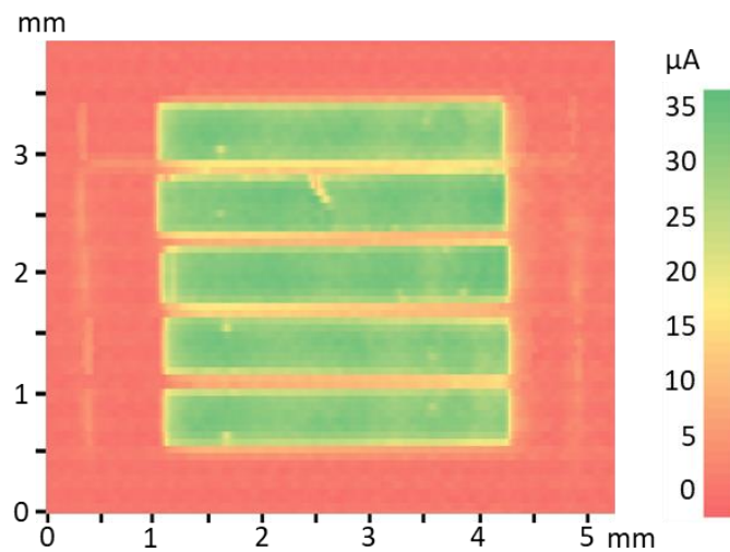
Figure 7. Map of the photosignal, as a result of scanning using the CW 3 \mu\text{m} laser spot of the Gaussian-like radiation distribution with the 1/e^2 diameter of 260 \mu\text{m} .
