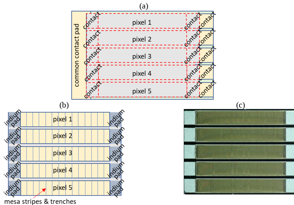
Figure 2. Linear array layout: (a) chip-on-carrier top view with: the delineation of pixels and contact pads, a single pixel area of 3.2 mm x 0.5 mm, pixels separated by a 0.1-mm gap, yellow indicating the gold contact pads on the carrier, contact pads in grey indicating the indium contact pads under chip, a carrier of 5 mm x 3 mm, and a chip of 4 mm x 3 mm; (b) view of the metallized HgCdTe side of the chip, with: the delineation of pixels, indium contact pads, and mesa structures of multiple photovoltaic micro-cells connected in series between indium pads; (c) micrograph of the same metallized side of the chip.
