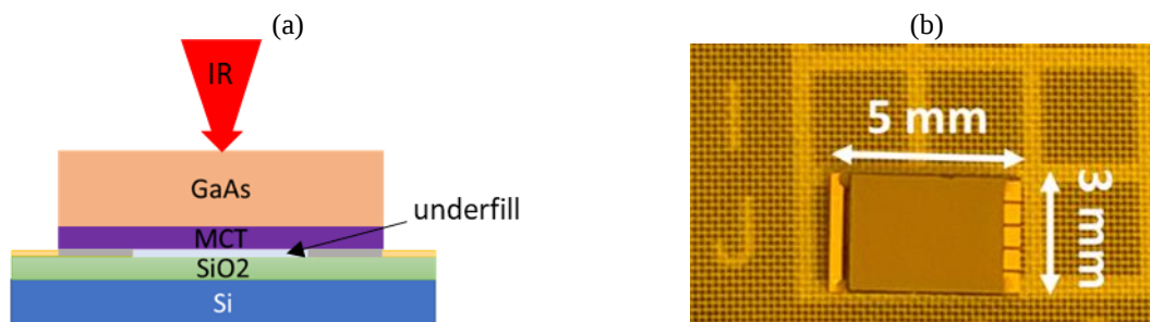
Figure 1. (a) Linear array cross-section, with direction of the infrared (IR) illumination; (b) chip-on-carrier micrograph top view, with a common contact pad on the left and individual pixel output contact pads on the right.
