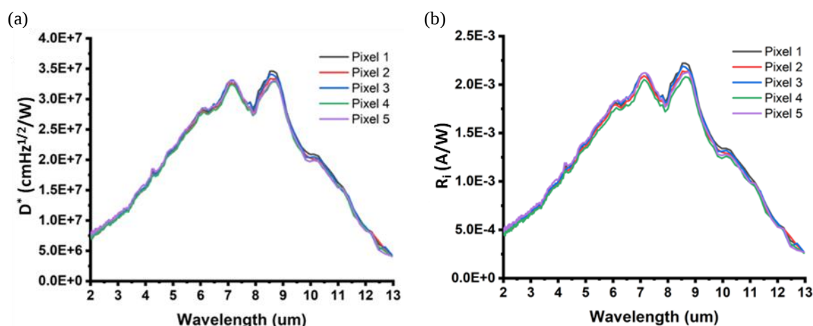
Figure 8. Example spectral characteristics of individual pixels: (a) detectivity, (b) responsivity.
