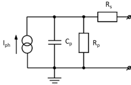
Figure 5. Equivalent small signal circuit of an individual pixel.
