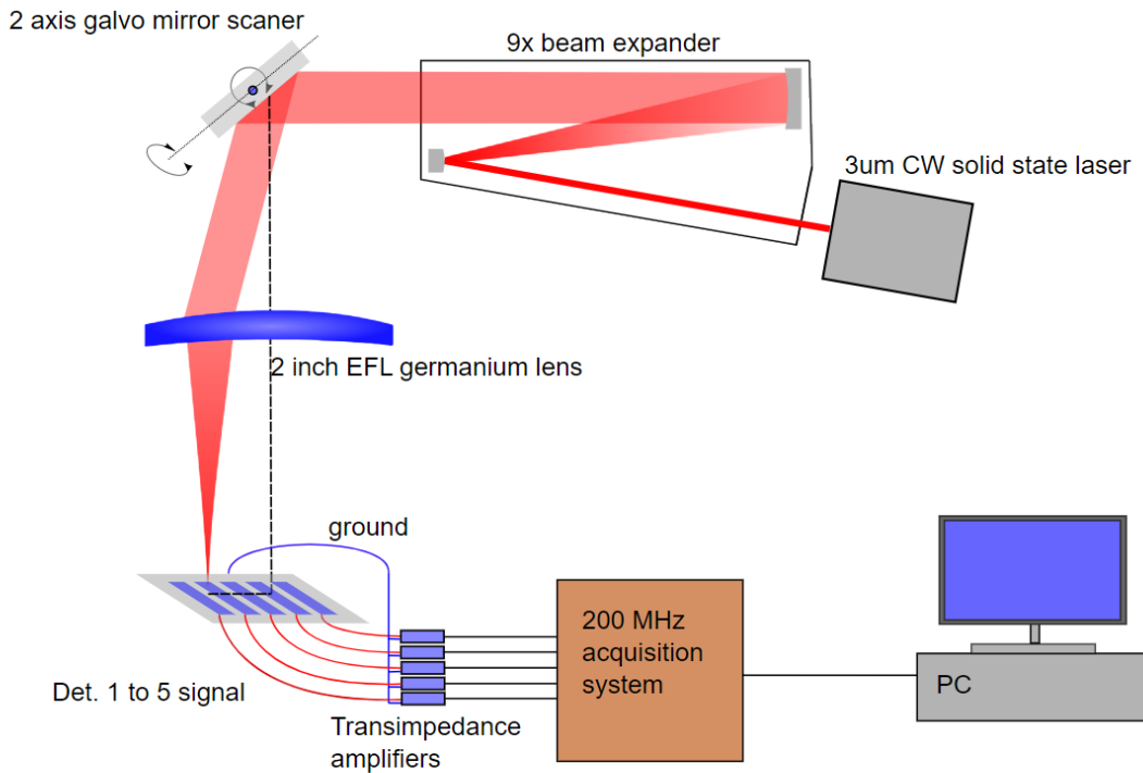
Figure 6. Measurement setup for mapping a photosignal across a linear array.
