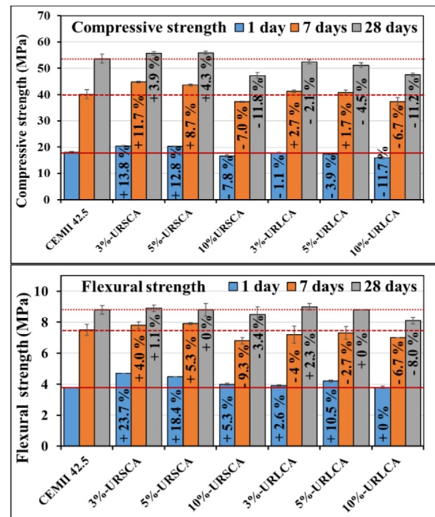
Fig. 11. Compressive and flexural strength of mortar pastes blended with ultrafine recycled concrete additions.
