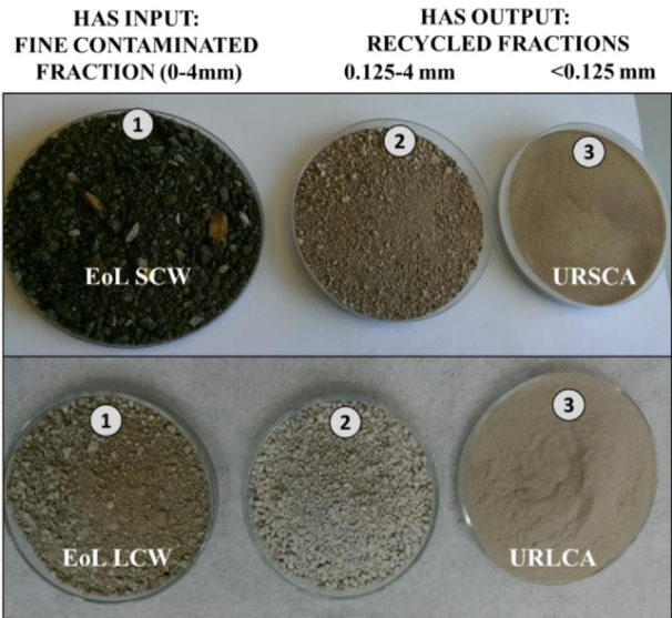
Fig. 4. (1) HAS input. (2&3) HAS recycled fractions.
