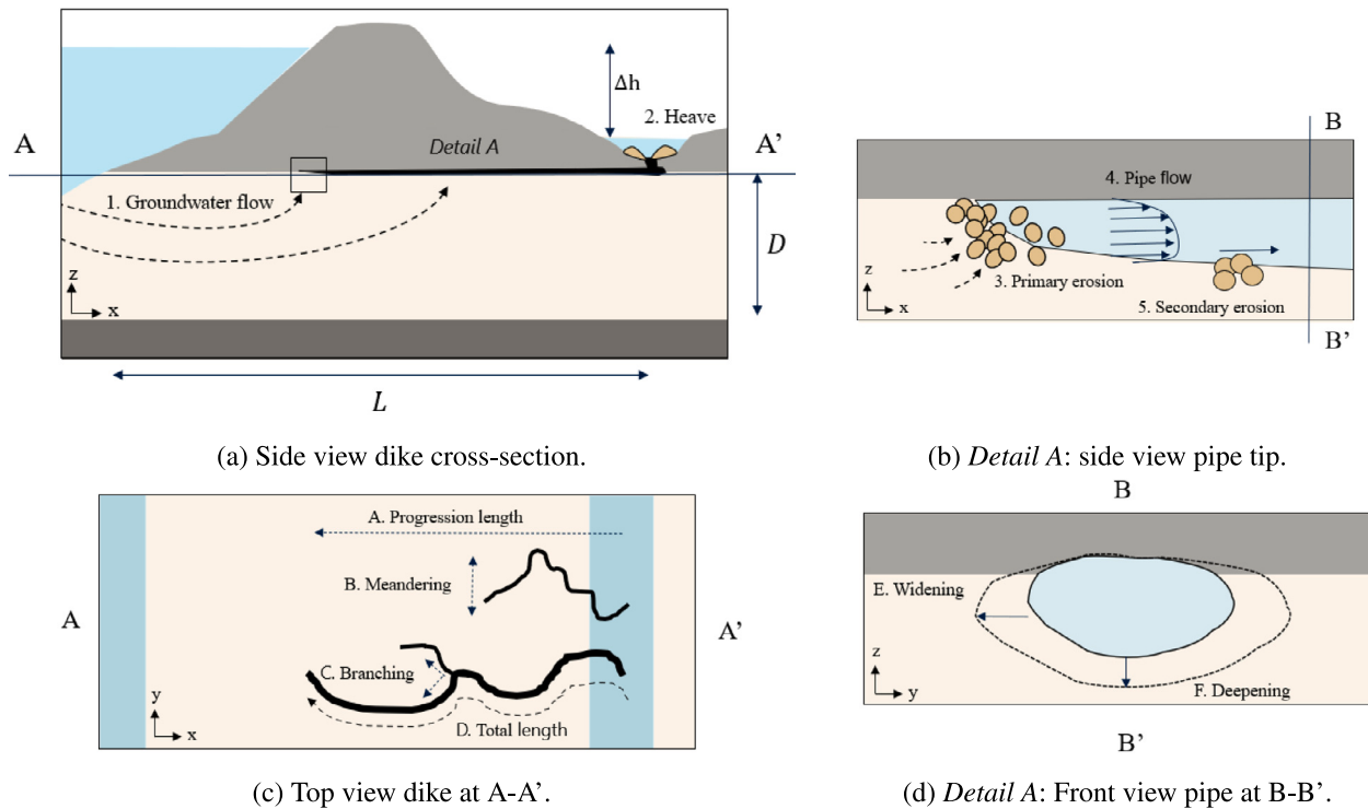
Fig. 1. Backward Erosion piping is governed by the physics shown in (a) and (b). Groundwater flow towards the pipe and outlet (1) leads to the heave at the outlet (2) if no pipe is present or the removal of sediments at the pipe tip if a pipe has started to form (3). The flow inside the pipe (4) leads to the removal of sediments from the bottom and walls of the pipe (5). The morphology of the pipe is shown in (c) and (d). The progression length is the distance (from downstream to upstream) the pipe has grown (A). The pipe meanders through the soil (B) if the pipe splits up and/or merges again, this is called branching (C). The total length of the pipe is the length along the entire pipe path (D) and due to secondary erosion, the pipe widens (E) and deepens (F).
