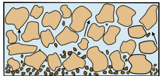
(c) Internal instability/suffusion
