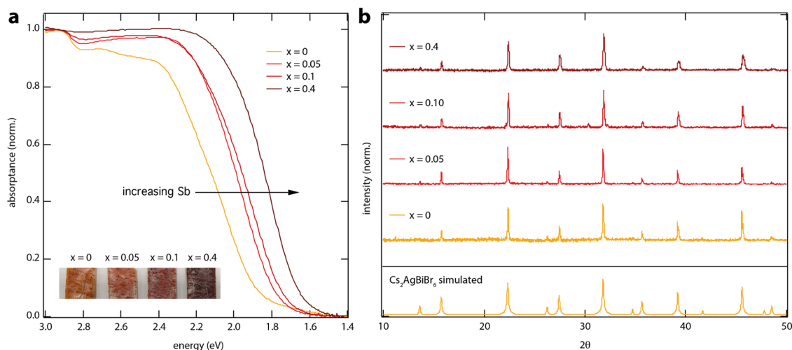
Figure 1. (a) Absorbance spectra normalized to unity to account for different surface coverages and (b) powder X-ray diffraction (XRD) patterns (Cu K \alpha radiation, \lambda = 1.54 Å) of mixed antimony–bismuth HDP powders with the general formula \text{Cs}_2\text{AgBi}_{1-x}\text{Sb}_x\text{Br}_6 . Inset shows images of the powders with different Sb content.
