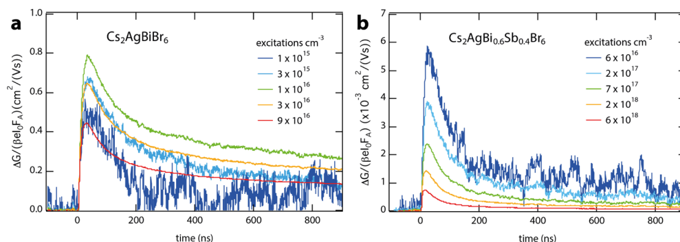
Figure 4. Photoconductance as a function of time after excitation at 2.8 eV for \text{Cs}_2\text{AgBiBr}_6 (a) and \text{Cs}_2\text{AgBi}_{0.6}\text{Sb}_{0.4}\text{Br}_6 (b).
