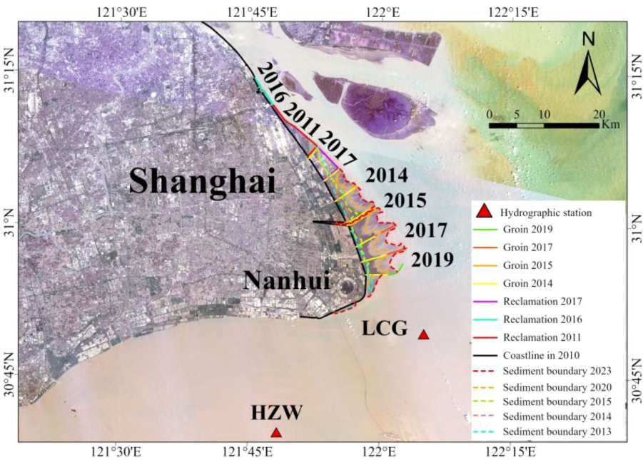
FIGURE 14 The Nanhui siltation promotion project and the changes of the sediment boundaries since 2010.
