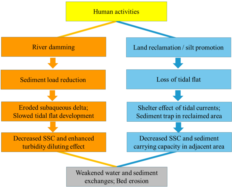
FIGURE 15 Conceptual model depicting the sediment dynamic response to human activities in the transitional zone between the Changjiang Estuary and Hangzhou Bay.
