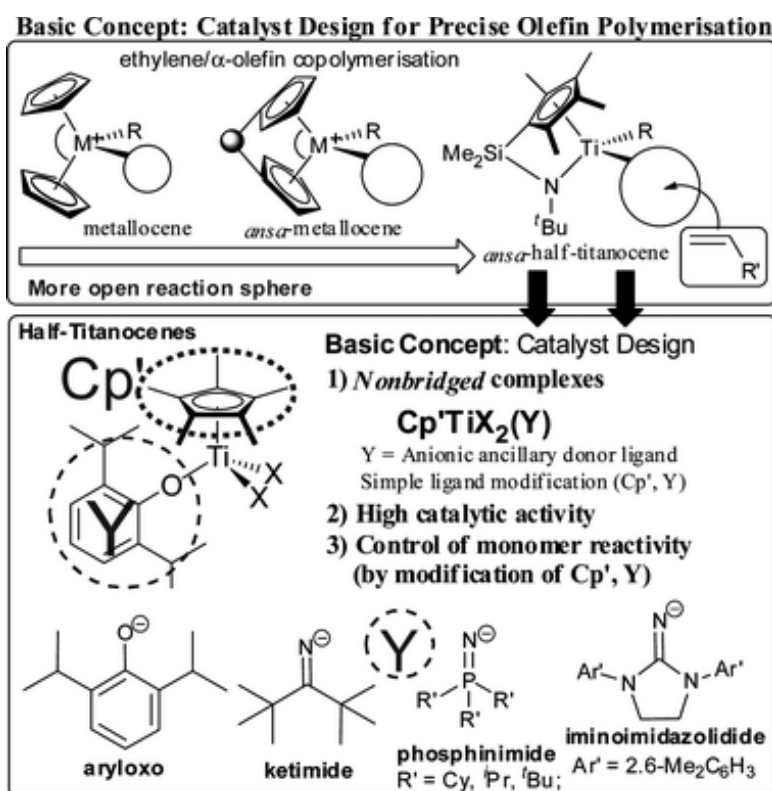
Scheme 1. Basic proposed concept for the catalyst design and selected examples for half-titanocenes as effective catalyst precursors for olefin polymerization, reprinted with permission from [3]. Copyright 2013 World Scientific.
