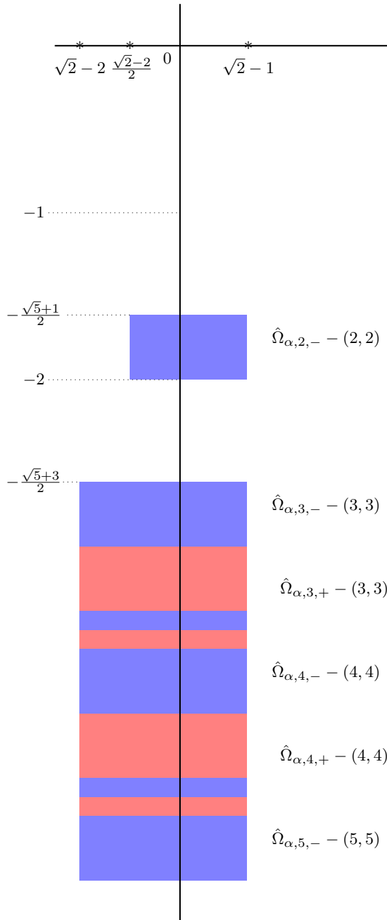
Figure 3. \Omega_\alpha^* for \alpha = \sqrt{2} - 1
