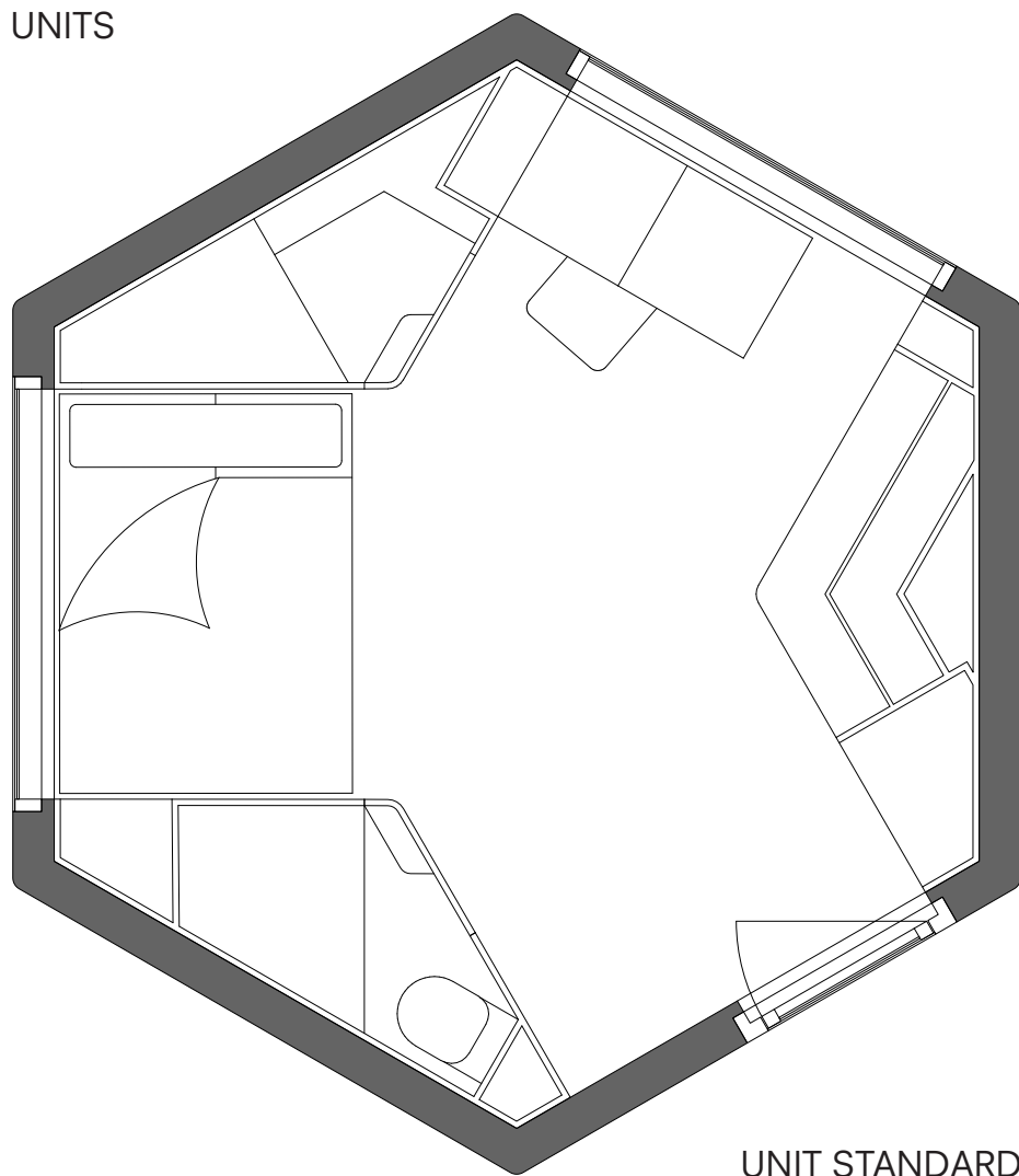
UNIT STANDARD
