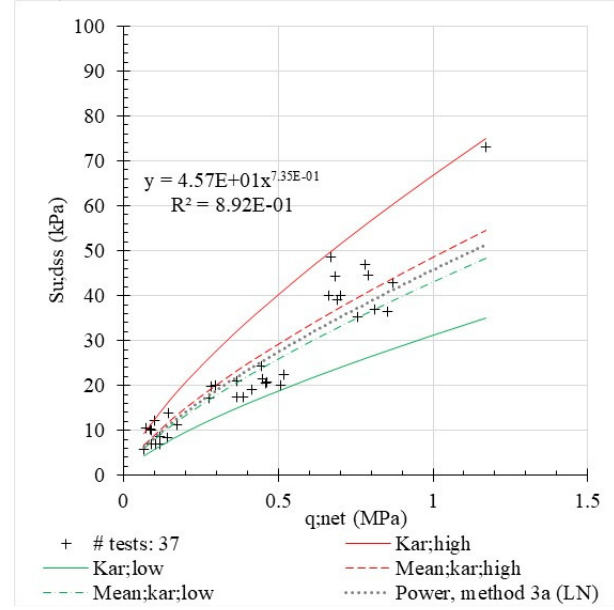
Figure 10. Method 3a, power function, OLS regression, LN transformation.
