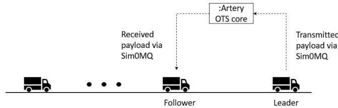
Figure 1: OTS-Artery architecture showing information exchange between a leader-follower pair and the Artery OTS core. The follower then calls the core upon message reception and receives the payload if the follower id matches the receiver GTU id in the payload. A new payload is transmitted every 100 ms. More information about OTS-Artery is available at: https://github.com/salilrsharma/OTS-Artery .
