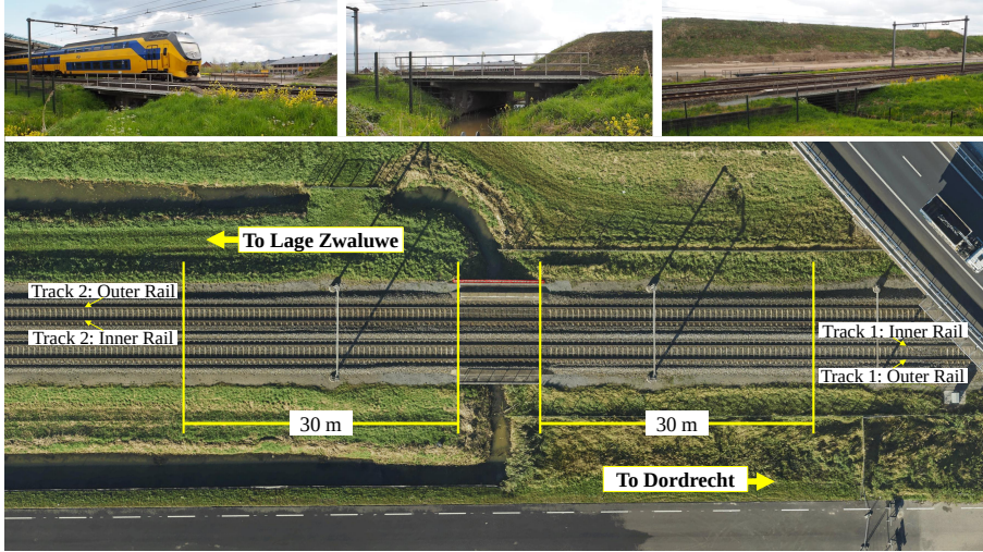
(a) Photographs at the double-track railway bridge across a water channel from the side and top view.
