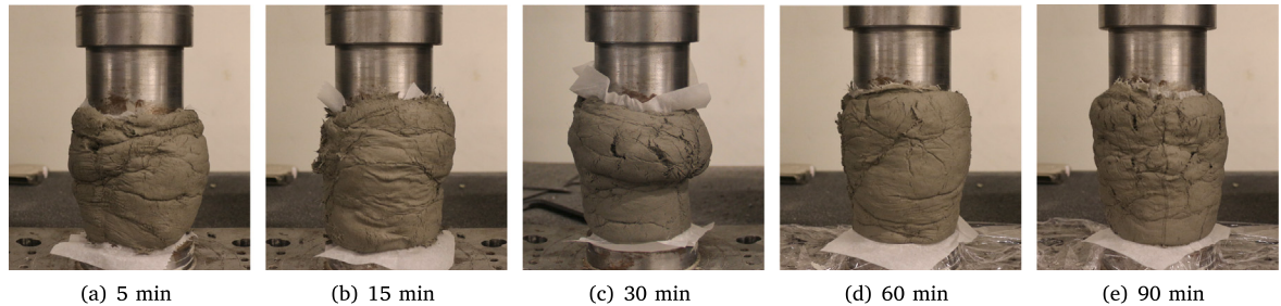
Fig. 7. Images of UUCT for Mix A of different ages with a constant vertical strain of 27.8%.
