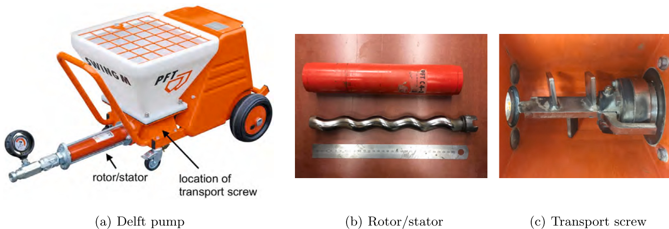
Fig. 18. Pump configuration.
