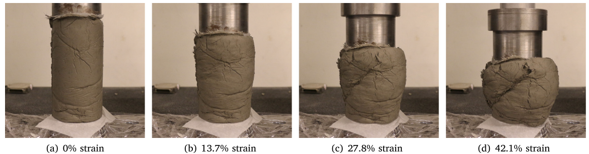
Fig. 6. Images of UUCT for Mix A (60 min) with increasing vertical strain.
