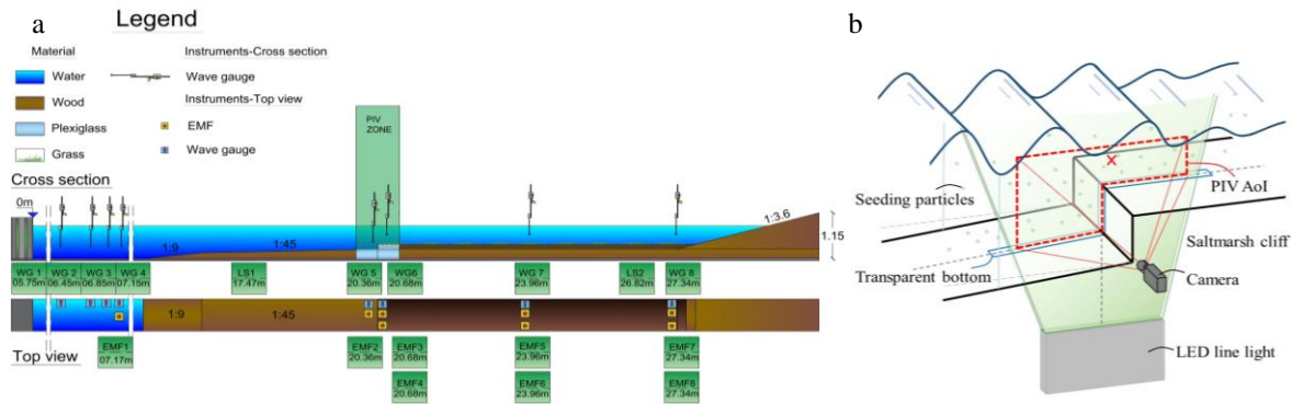
Figure 1. Schematic overview of wave flume setup (a), with detailed overview of the PIV setup at the saltmarsh cliff (b).
