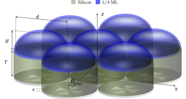
Fig. 1. The schematic of the proposed hexagonally oriented dual-polarized leaky lens antenna array.
