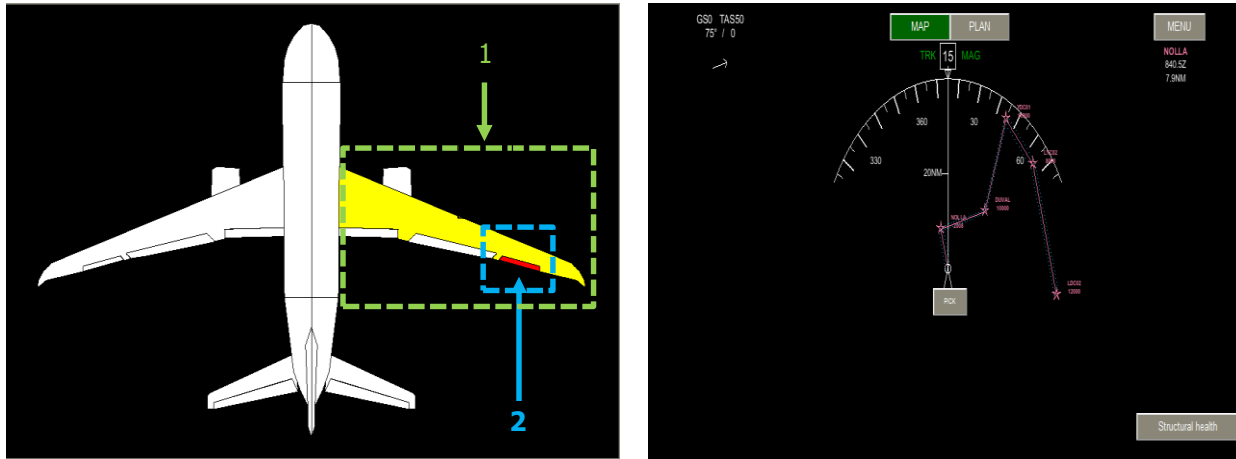
Figure 5. a) Example of how inflight structural health monitoring could be combined with visualisation tools. Region 1 is a warning indication of medium damage to wing and region 2 indicates large structural damage to the aileron. b) Example of a multi-functional display [17, 18] which would be used to present SHM data to the pilot, in combination with acoustic warning.
