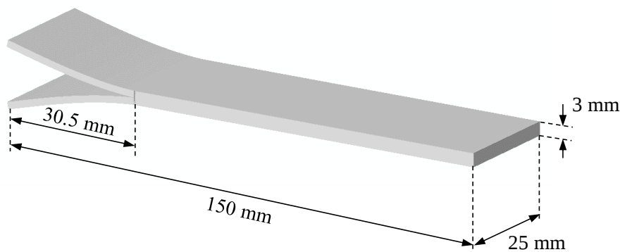
Figure 4: DCB specimen geometry.
