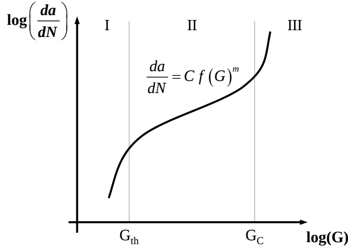
Figure 1: Typical fatigue crack growth curve.
