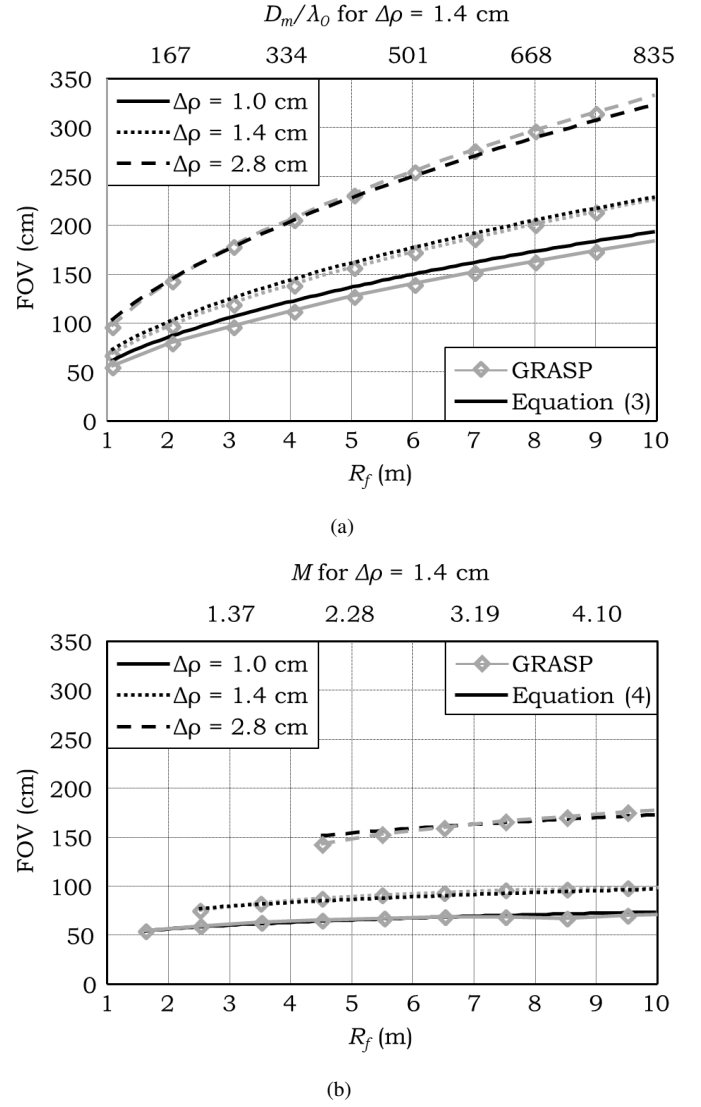
Fig. 4. Effective FOV as a function of the imaging distance for the described canonical reflector architectures: (a) symmetric elliptical reflector, (b) symmetric confocal dual-reflector.
