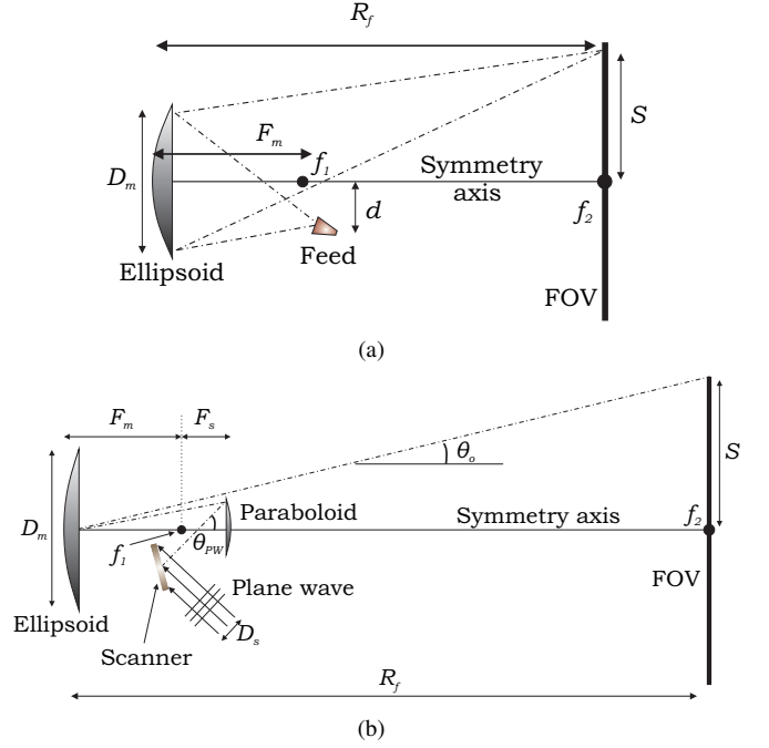
Fig. 3. Canonical reflector geometries considered in the analysis: (a) symmetric elliptical reflector and (b) symmetric confocal dual-reflector.
