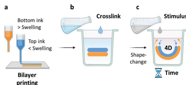
Figure 1. 4D printing concept based on swelling-based differential growth. a) A schematic drawing of the two inks 3D printed into a bilayer: high swelling (bottom layer, in orange) and low swelling (top layer, in blue). b) The scaffold is then crosslinked to obtain a solid construct. c) Finally, a swelling-based stimulus is applied on the construct, which triggers the construct's shape-based transformation behavior over time (4D).
