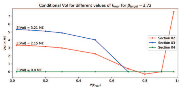
Figure 4. Conditional Value of Information for various values of k_{repr} for monitoring at different sections. P(k_{repr}) denotes the non-exceedence probability of k_{repr} after monitoring. A small P(k_{repr}) denotes a very favorable monitoring outcome. E(Vol) denotes the Vol weighted by the scenario probabilities. The Vol is here the difference in investment cost to segment a certain target reliability \beta_{target} compared to the investment cost without monitoring.
