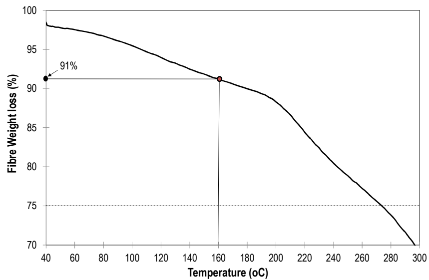
Figure 9 Sodium Alginate Compartmented fibres containing rejuvenator TGA test results.
