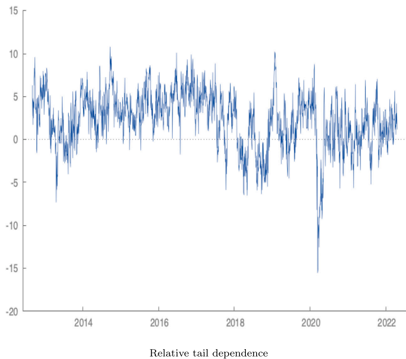
Fig. 12. Relative tail dependence ( TCI_{\tau_{0.90}} - TCI_{\tau_{0.10}} ). Note: This figure displays the time-varying difference between the TCI at the 90th quantile and the TCI at the 10th quantile, with both indices estimated based on 100 days window length and a forecast horizon of 10.
