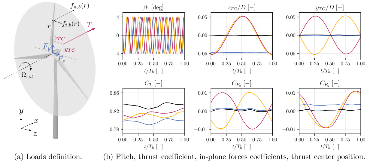
Figure 2. (a) Schematic representation of resulting in-plane forces ( F_{y,z} ) and out-of-plane force ( T ). (b) Evolution of pitch angle and forces over one helix period T_h for BL (—), ST (—), CCW (—), CW (—). All force-related signals are notch-filtered at 3P for clarity purposes and forces are made dimensionless following C_* = */ \left( 0.5 \rho U_{ref}^2 \pi R^2 \right) , * = T , F_y or F_z .
