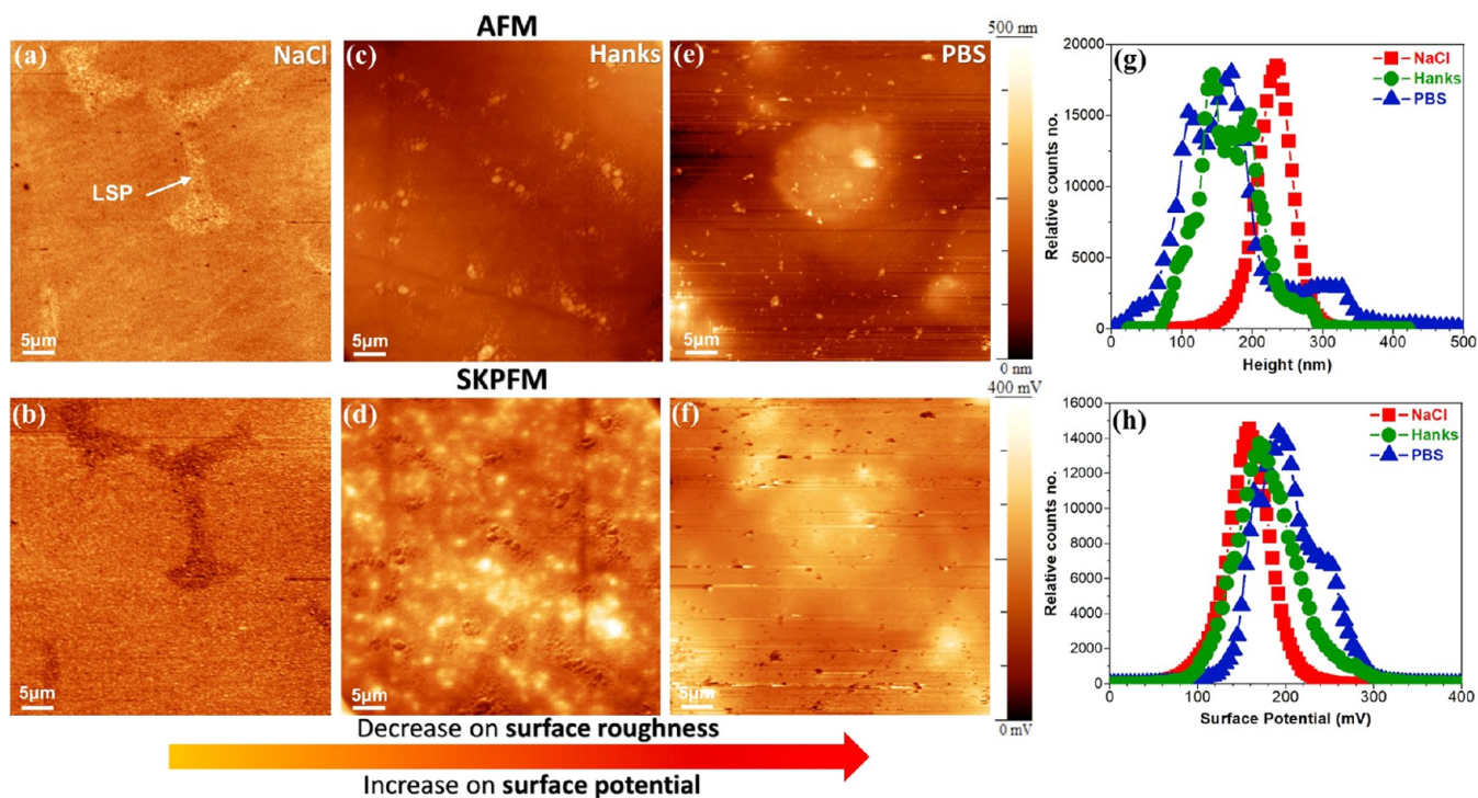
Figure 8. AFM (first row) and SKPFM (second row) images of the WE43 Mg-based alloy after 10 min of immersion in (a, b) 0.9% NaCl, (c, d) Hanks's, and (e, f) PBS physiological solutions at 37 °C, pH 7.4, and aerated conditions. (g) Height and (h) surface potential histograms that are related to SKPFM images in (b), (d), and (f).
