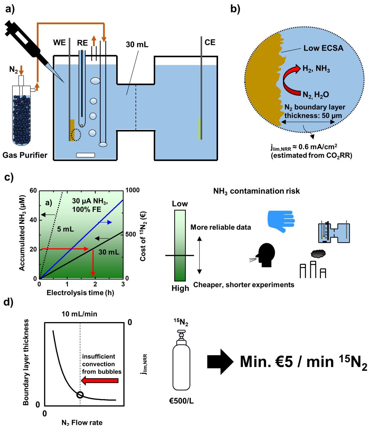
Figure 1. Limitations of H-cell design for NRR studies. (a) Schematic of an H-cell and gas purification. (b) Schematic of the electrode surface with 50 μm boundary layer and resulting mass-transport limiting current for NRR j_{lim,NRR} . (c) Dependence of the accumulated NH 3 and the cost of an isotope labeling experiment on the electrolysis time and the electrolyte volume. Ammonia production from NRR: 30 μA, flow rate during 15 N 2 experiments: 10 mL/min. The green color gradient represents the risk of NH 3 contamination (summarized from Table S2). (d) Dependence of N 2 mass transport to the cathode on the N 2 flow rate and resulting minimal cost of isotope labeling. Adapted from ref 26. Copyright 2018 American Chemical Society.
