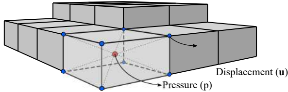
Figure 5.1: Computational grid for pressure and displacement used in FEM-FVM solver highlighting pressure in the center and displacement nodes in the corner.
