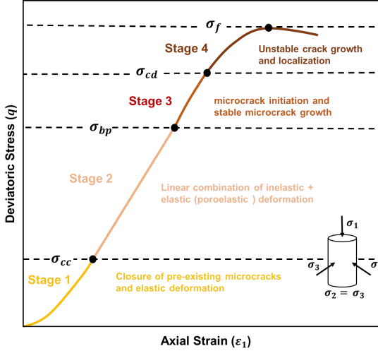
Figure 4.1: Stress-strain curve showing deformation stages of Red Felsler sandstone under the condition of constant confining pressure (10 MPa). The four stages of stress levels are: the initial crack closure ( \sigma_{cc} ), brittle yield point stress ( \sigma_{bp} ), crack damage stress ( \sigma_{cd} ) and maximum strength ( \sigma_f ).
