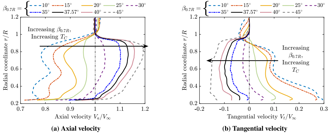
Fig. 20. Radial distributions of time-averaged axial and tangential velocity in the propeller slipstream at 1R downstream of the propeller center at J = 1.34 .
