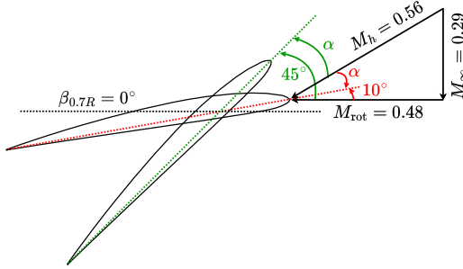
Fig. 15. Velocity triangle for the constant operating condition ( J = 1.34 ) at different pitch settings at r/R = 0.7 (ignoring induction).
