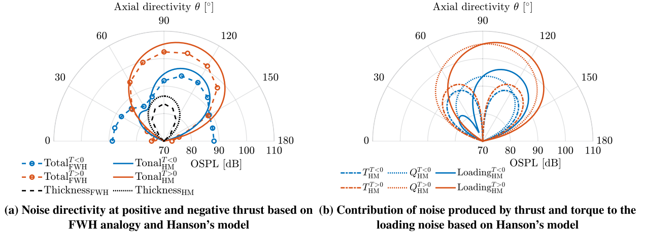
Fig. 21. Far-field noise directivity of the propeller in positive and negative thrust regimes at absolute thrust level of |T_C| = 0.08 at J = 1.34 .
