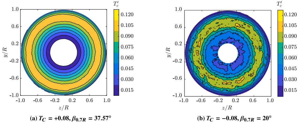
Fig. 16. Radial distribution of instantaneous thrust coefficient ( T'_c ) along the propeller blade span over a rotation as a function of circumferential position for T_C = \pm 0.08 at J = 1.34 .
