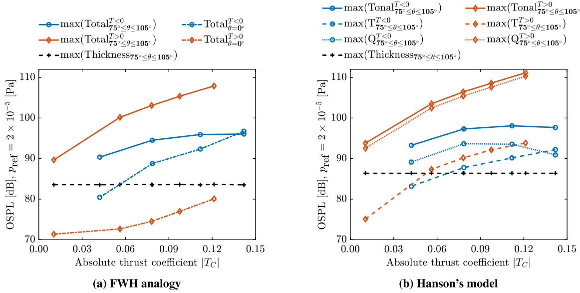
Fig. 25. Effect of thrust coefficient on the noise sources in positive and negative thrust regimes for a propeller operating at a constant rotational speed ( J = 1.34 ).
