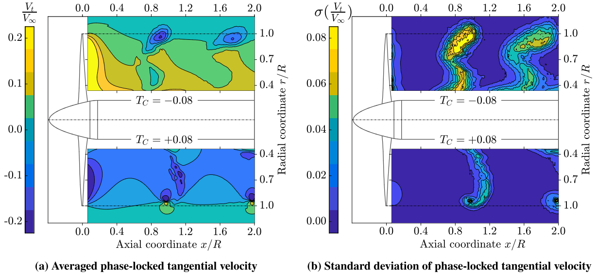
Fig. 19. Comparison of tangential velocity contours in negative ( \beta_{0.7R} = 20^\circ ) and positive ( \beta_{0.7R} = 37.57^\circ ) thrust condition at absolute thrust level of |T_C| = 0.08 (Phase-locked).
