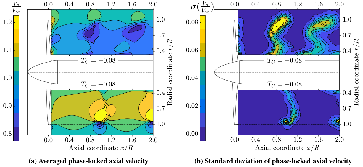
Fig. 18. Comparison of axial velocity contours in negative ( \beta_{0.7R} = 20^\circ ) and positive ( \beta_{0.7R} = 37.57^\circ ) thrust condition at absolute thrust level of |T_C| = 0.08 (Phase-locked).
