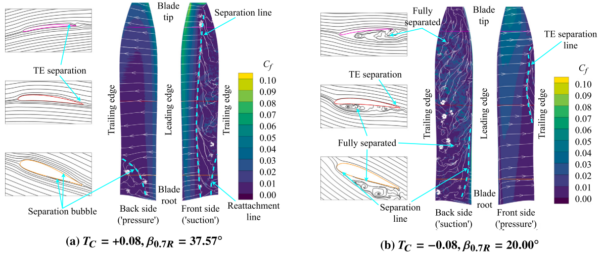
Fig. 13. Visualization of instantaneous flow around the propeller blade using skin friction coefficient and shear lines for T_C = \pm 0.08 at J = 1.34 .
