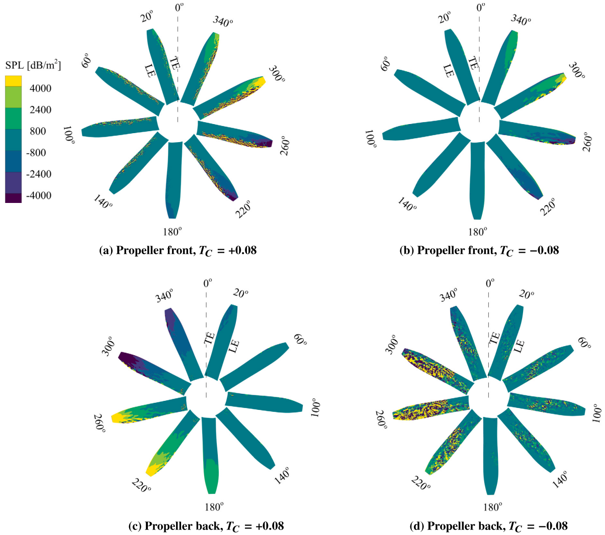
Fig. 24. Noise source map (1st BPF) on a single propeller blade for an observer located in the propeller plane ( \theta = 90^\circ ) at positive and negative thrust conditions at J = 1.34 .
