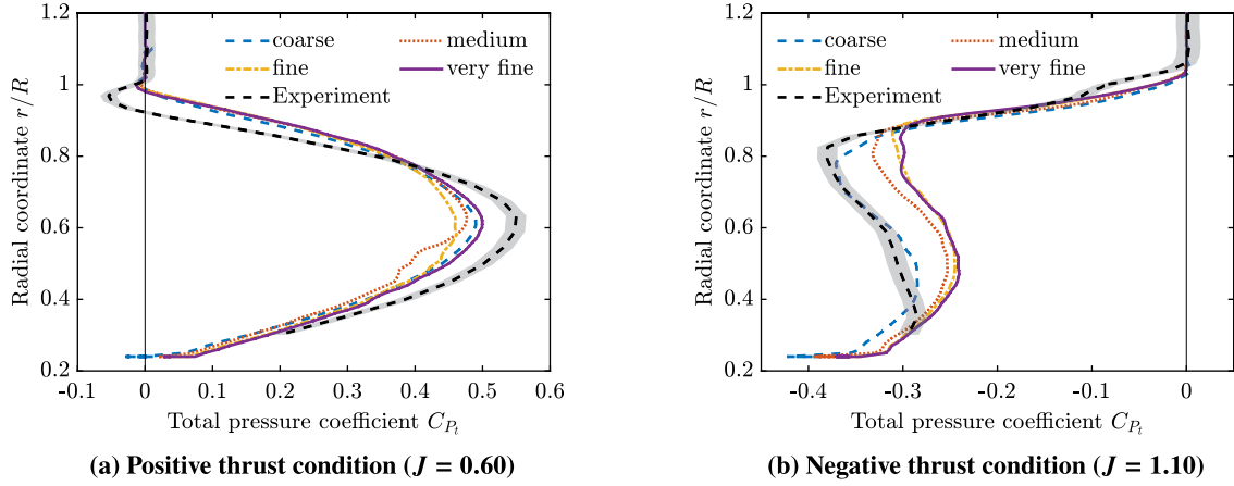
Fig. 6. Radial distributions of time-averaged total pressure coefficient at 0.15R downstream of the propeller center.
