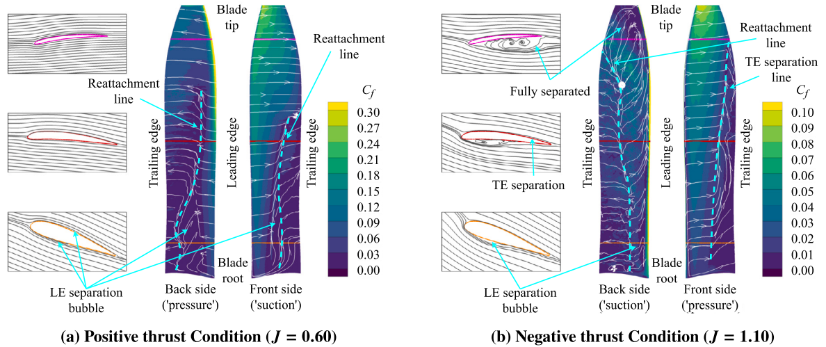
Fig. 5. Visualization of flow around the propeller blade using skin friction coefficient and shear lines (fine grid). (For interpretation of the colors in the figure(s), the reader is referred to the web version of this article.)
