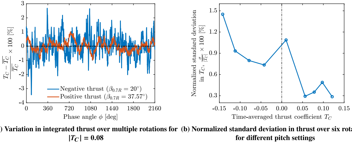
Fig. 17. Time-accurate integrated thrust performance at J = 1.34 .
