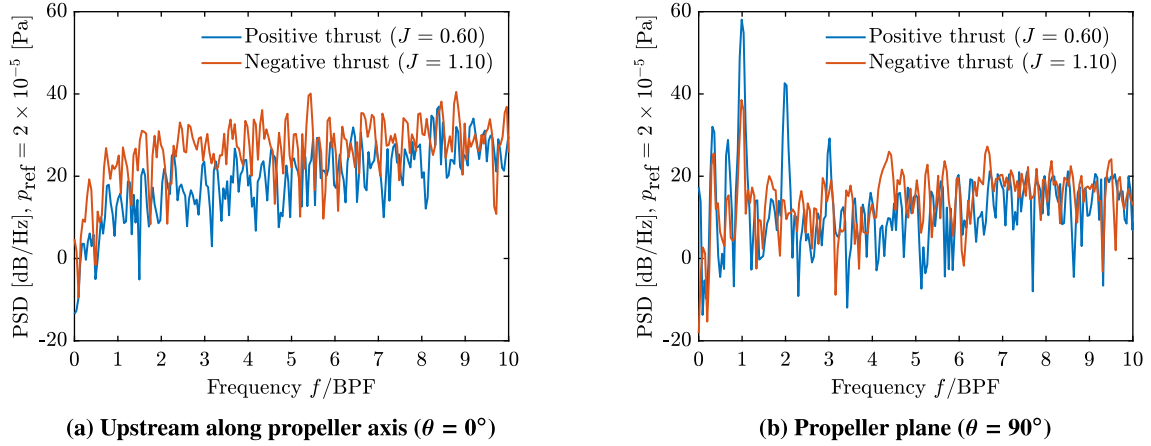
Fig. 12. Power spectrum density at \theta = 0^\circ and 90^\circ for positive thrust and negative thrust conditions (fine grid).
