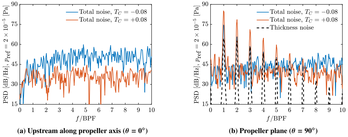
Fig. 22. Power spectrum density at \theta = 0^\circ and 90^\circ for absolute thrust level of |T_C| = 0.08 at J = 1.34 .
