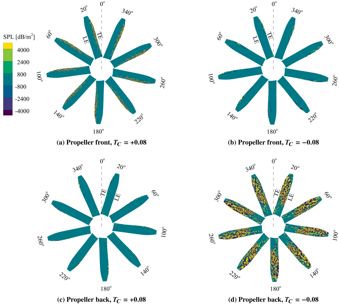
Fig. 23. Noise source map (1 - 2 BPF) on a single propeller blade for an observer located along the propeller axis ( \theta = 0^\circ ) at positive and negative thrust conditions at J = 1.34 .
