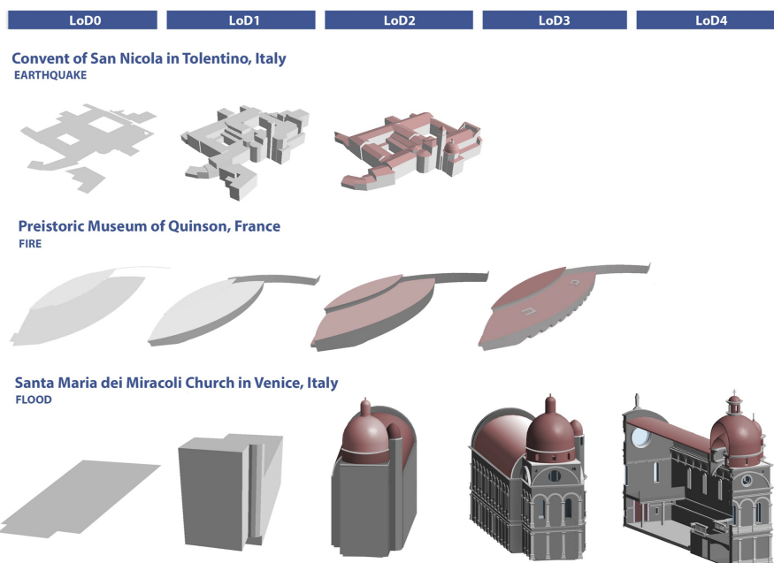
Figure 6. Examples of the used LoDs with the buildings of the three case studies
