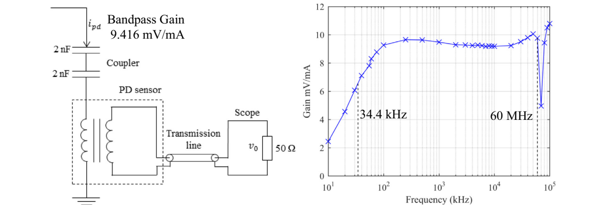
Fig. 6. Detection circuit made out of the HFCT sensor terminated at 50 \Omega oscilloscope input. Frequency response of the PD sensor.
