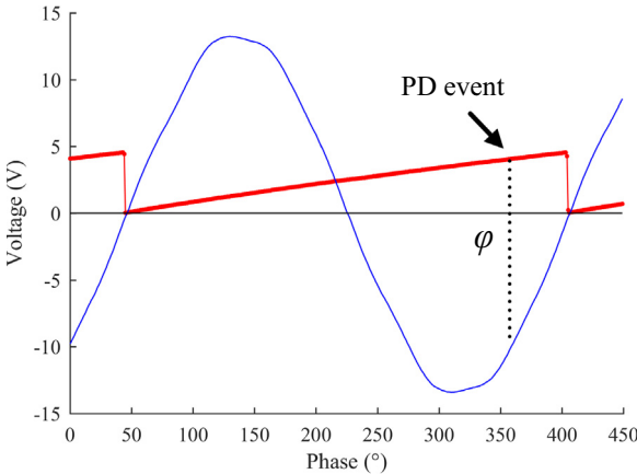
Fig. 8. Synchronization signal to acquire the phase of the PD pulses.
