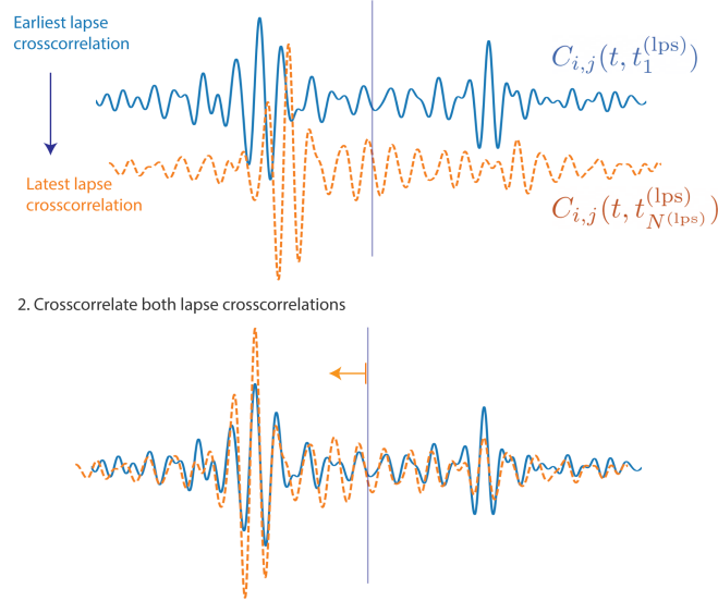
Figure 2 Processing steps for calculating an a priori estimate of the combined clock drift of a given station pair.
