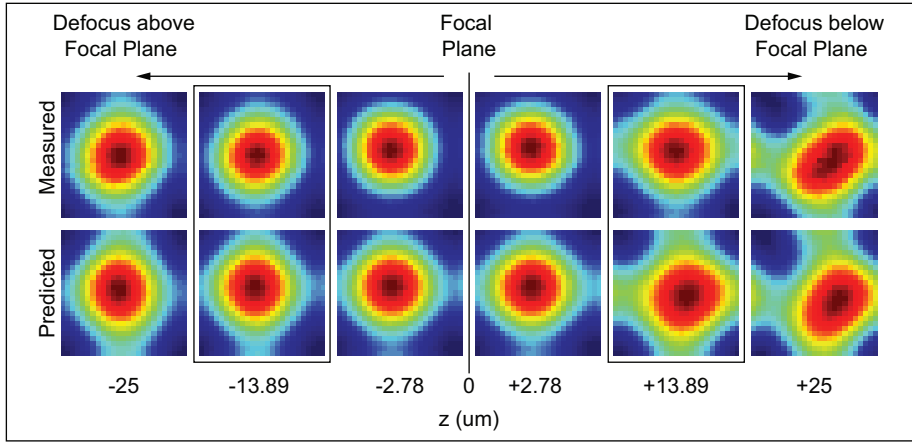
Figure 3.19: Comparison between the measurements and the predictions calculated using the retrieved 15 coefficients of aberrations. Unboxed figures are used for optimization while the boxed figures are not used.
