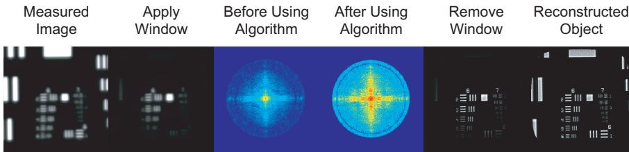
Figure 2.6: Flowchart of applying and removing the window function for the phase diversity method. In order to use the phase diversity algorithm, we need to apply the window function to the measured image and remove it from the reconstructed object (restored image). The removal is regularized by adding a small constant to the window function to avoid noise amplification.
