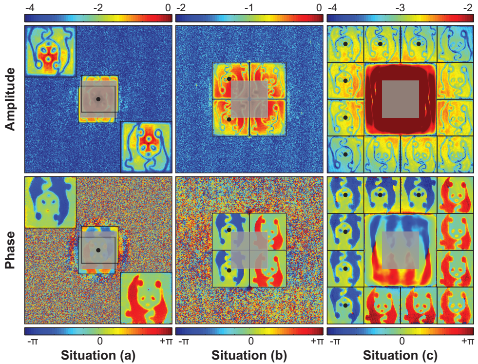
Figure 4.5: Experimental results of varying the perturbation point location for the GSM beam illumination. The gray square shows the aperture and the black dots show the perturbations points. In the phase plot, the red and the blue panda are the phase of the original object and its complex-conjugate, respectively. The panda contour in the amplitude plot is due to abrupt phase transition. The amplitude plot is in logarithmic scale. The quadratic term \hat{I}_0(\mathbf{x}) has been removed in (a) and (b). (c) is the direct inverse Fourier transform of the perturbed diffraction pattern.
