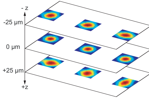
Figure 3.15: PSF-like images measured by three camera pixels (in three sub-regions) via scanning in three image planes. The FOV of the projection lens has a size of 32 \text{ mm} \times 55 \text{ mm} . Three PSF-like images, each with size of 4.5 \text{ } \mu\text{m} \times 4.5 \text{ } \mu\text{m} , can be measured simultaneously via one scanning process.
