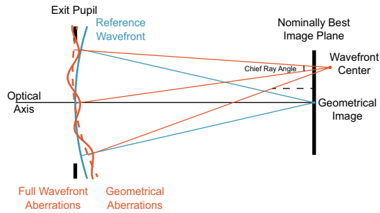
Figure 3.7: Schematic plot of the wavefronts at the exit pupil. The blue curve is the reference wavefront, which is a spherical wavefront with center at the geometrical image of the point source. The dashed and solid orange curves are the wavefronts affected by only tilt and defocus and by all aberrations, respectively.
