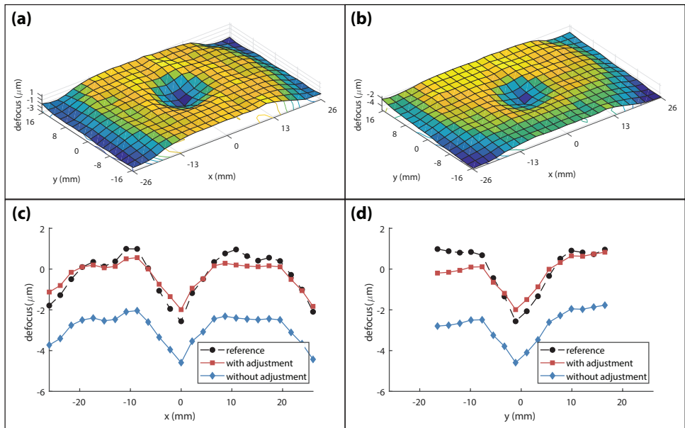
Figure 3.20: Comparison between the defocus aberration (field curvature) retrieved using our algorithm and the reference data in full FOV. (a) and (b) are the reference data and the retrieved field curvature, respectively. (c) and (d) are the x and y cross-sections of the plots in (a) and (b), respectively.
