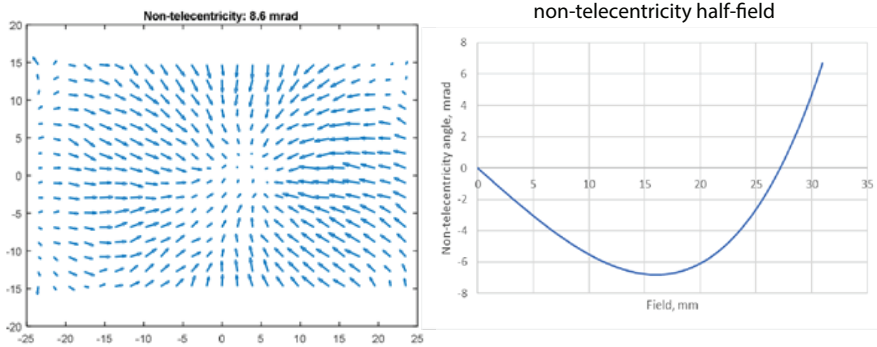
Figure 3.13: Results of telecentricity measurement. Left: experiment retrieval result. Right: ray tracing model simulation result along the x direction. The magnitude of non-telecentricity in the experimental retrieval result is given by the maximum chief ray angle.
