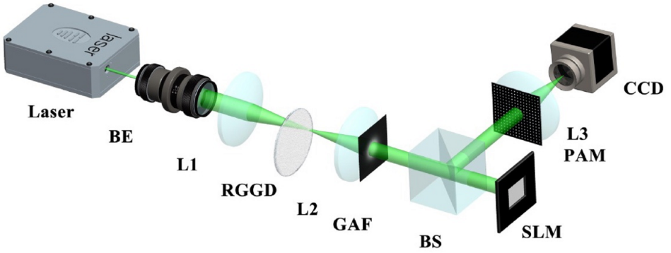
Figure 5.3: Experimental setup for Gaussian Schell-model beam generation and for diffractive imaging. BE: beam expander, RGGD: rough ground glass disc, GAF, Gaussian amplitude filter, BS: beam splitter, SLM: spatial light modulator, PAM: pinhole array mask, and L1,L2,L3 are thin lenses.
