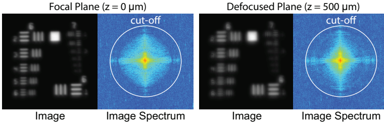
Figure 2.3: Resolution target and measurements of two through-focus images in spatial domain and spatial frequency domain. Group 6 and group 7 of the resolution target are imaged by a CCD camera located in the nominal image plane at z = 0 and a defocused plane at distance z = 500 \mu\text{m} .
