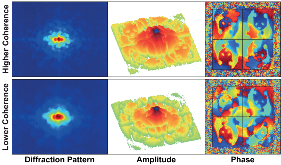
Figure 4.8: Diffraction pattern and the inverse Fourier transform for GAC beam illumination with two degrees of coherence. The transmissive object is superposed with the aperture.
