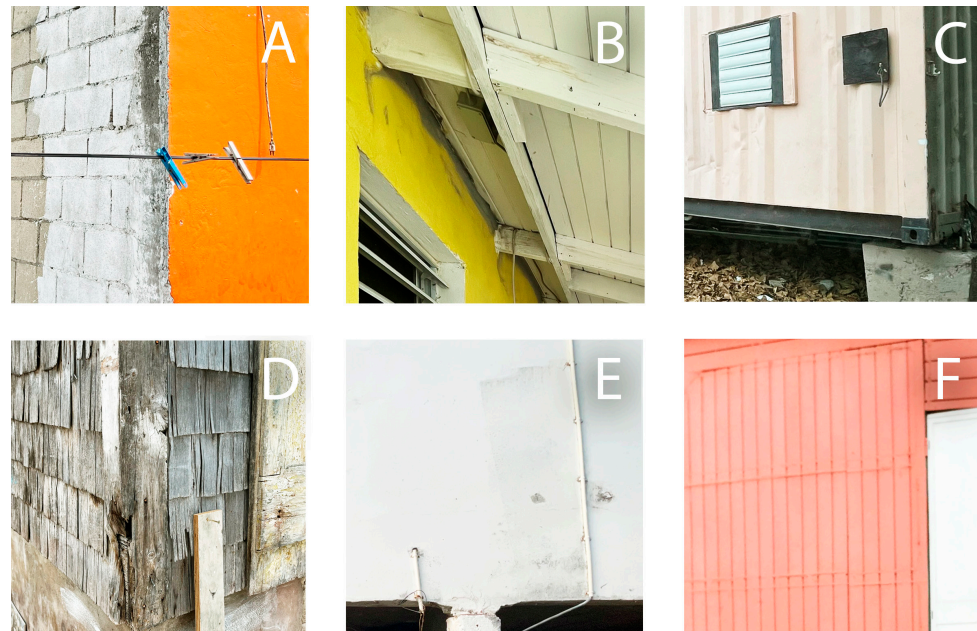
Figure 7. Building materials used for a structure: (A) concrete blocks; (B) concrete wall and timber rafters; (C) container on poured concrete pillar. Materials used for the skin: (D) wooden shingles; (E) cement; (F) wooden cladding.
