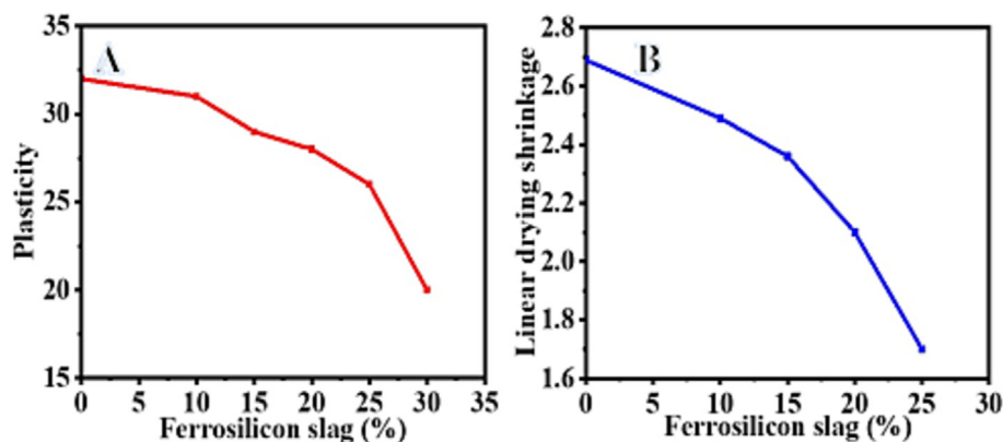
Fig. 3. The influence of FS addition on the Plasticity (A) and dry shrinkage (B).
