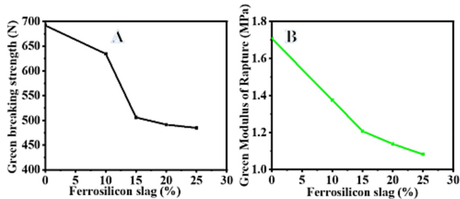
Fig. 4. The influence of FS addition on the green breaking strength (A) and green Modulus Of Rapture (B).
