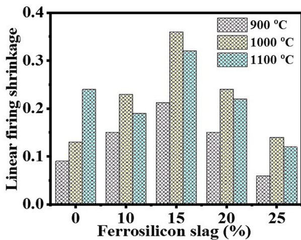
Fig. 5. The influence of FS slag addition and firing temperatures on linear firing shrinkage.
