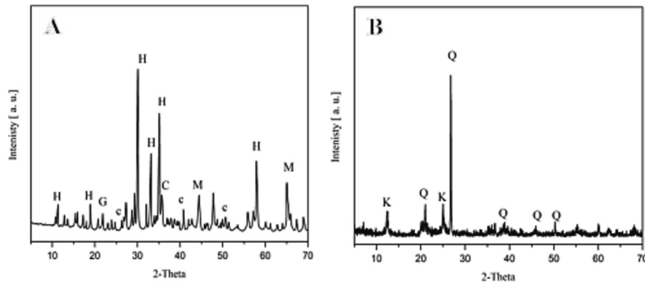
Fig. 2. XRD Analysis of FS slag (A); H. Hexagonal alumina, C. Cryolite, c. rhombohedral corundum, G. goethite and XRD Analysis of kaolin clay (B); K. kaolinite, Q. quartz.
