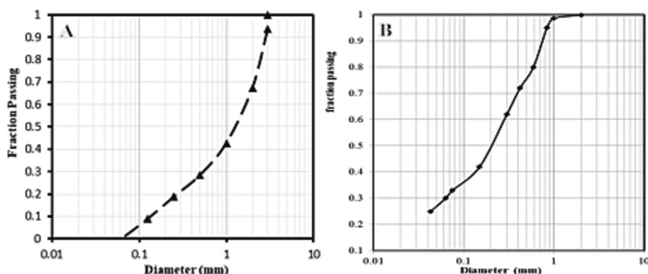
Fig. 1. Particle size distribution of raw materials (A) clay and (B) FS slag.
