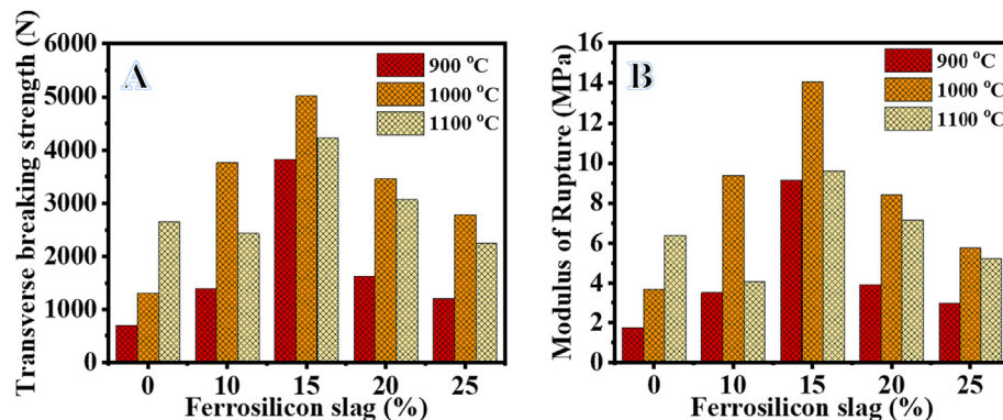
Fig. 6. The influence of FS slag addition and firing temperatures on TBS (A) and MOR (B).
