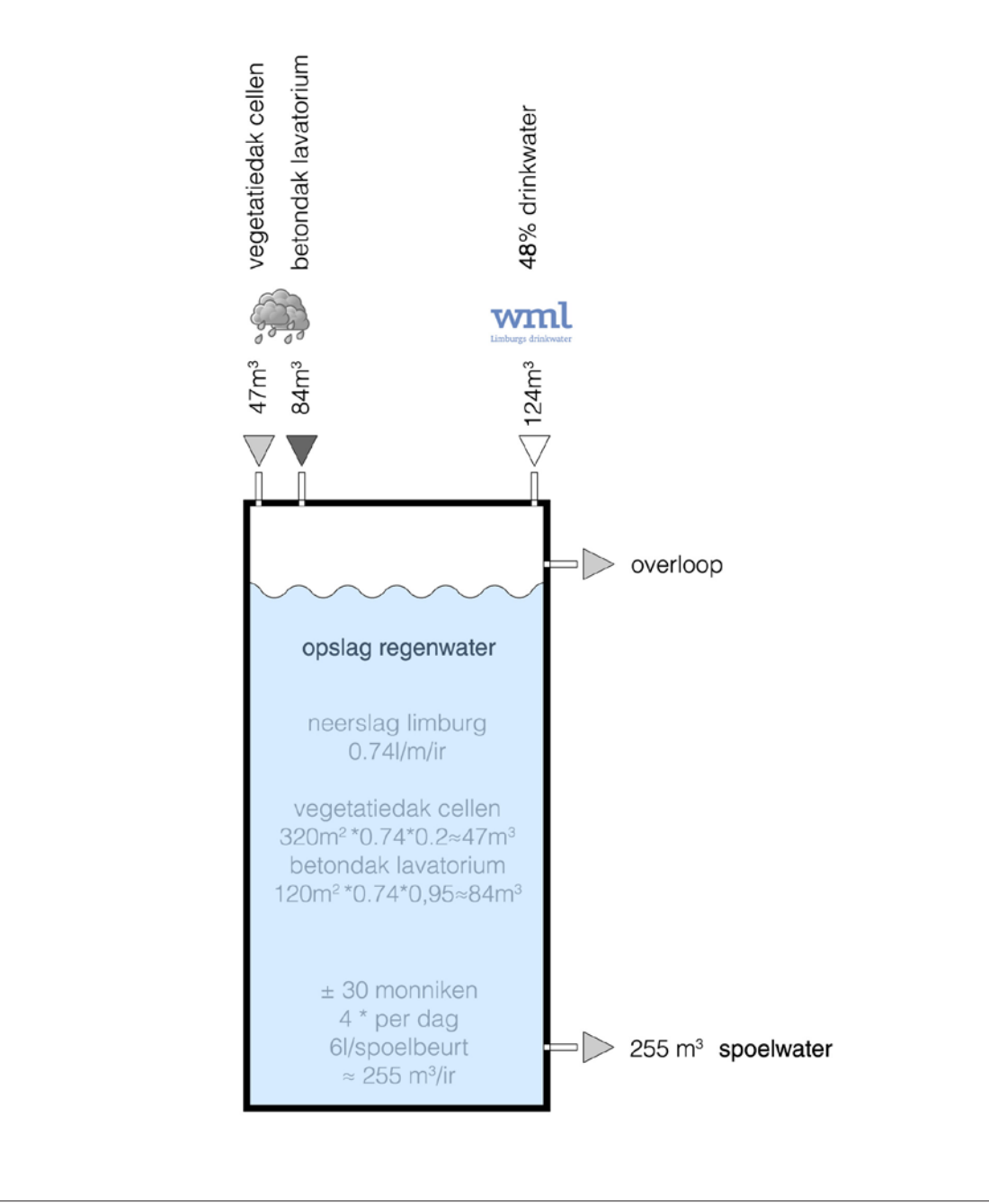
SCHEMA WATER
