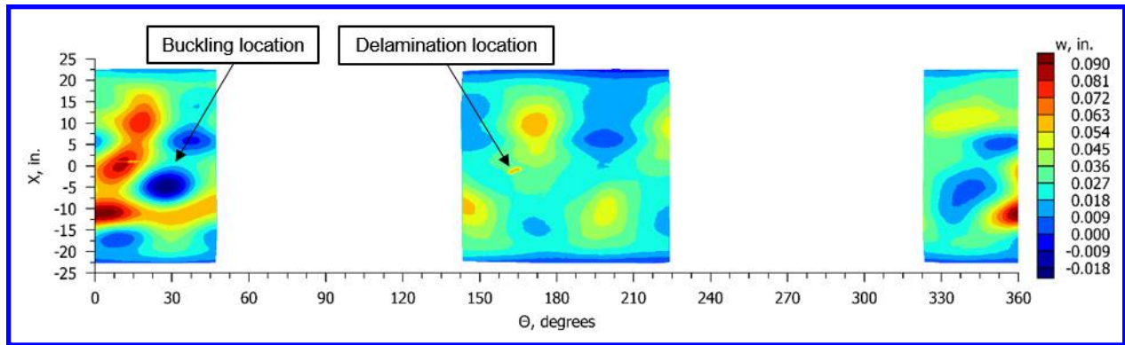
a.) Radial displacements.
