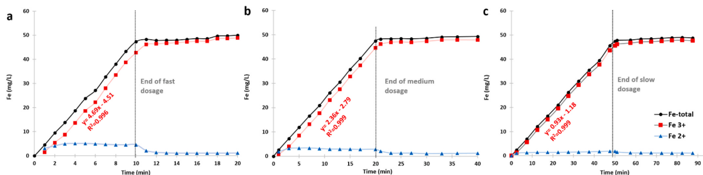
Fig. 8. Fe profiles (Total Fe, Fe 2+ and Fe 3+ ) during (a) fast dosage (b) medium dosage and (c) slow dosage. The best fitting linear equation and R 2 for the Fe 3+ series (during Fe supply) is indicated in each case, together with the timestamp in which Fe supply is stopped. All experiments were performed in duplicate.
