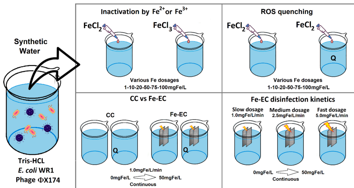
Fig. 3. Schematic description of the four Fe disinfection experiments. Letter “Q” indicates the beaker was dosed with an ROS-Quencher. Pipette represents single-event chemical dosage, while the arrow represents continuous dosage either by CC ( \text{FeCl}_2 solution dosed with peristaltic pump) or Fe-EC (Fe dosed electrochemically under a constant current).
