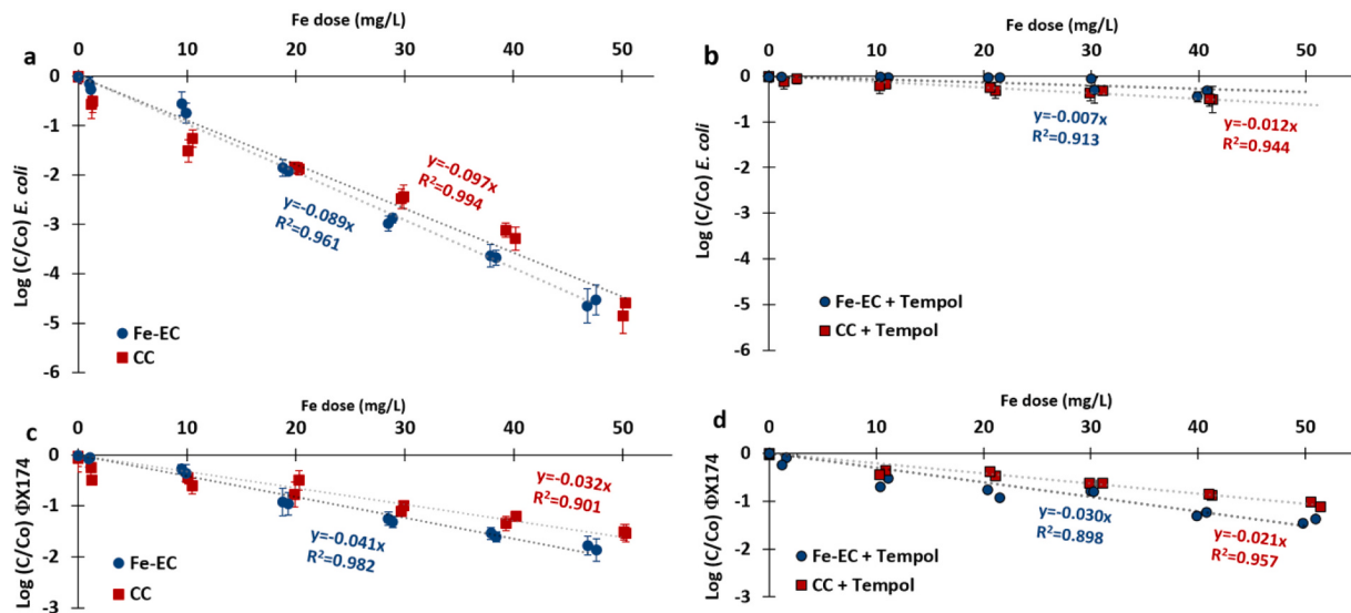
Fig. 6. Inactivation of E. coli under CC and Fe-EC without TEMPOL (a) and with TEMPOL (b), and inactivation of phage \Phi X174 under CC and Fe-EC without TEMPOL (c) and with TEMPOL (d). Error bars represent standard deviation. All experiments were performed in duplicate, and all microbial determinations were executed in triplicate.
