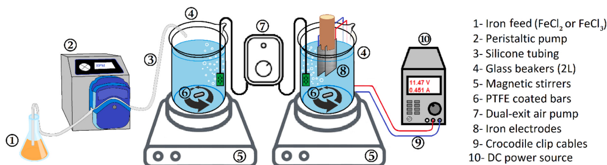
Fig. 2. Fe dosage bench scale setup, with chemical dosage (left) and electrochemical dosage (right).
