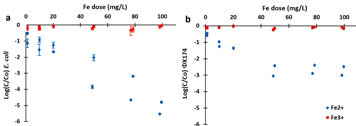
Fig. 4. Inactivation of (a) E. coli WR1 and (b) somatic coliphage \Phi\text{X174} during dosing 0–100 mg/l of either \text{Fe}^{2+} or \text{Fe}^{3+} . Error bars represent standard deviation. All experiments were performed in duplicate, and all microbial determinations were executed in triplicate.
