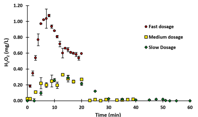
Fig. 9. Average H 2 O 2 production profiles during fast, medium and slow Fe dosage. All experiments were performed twice. Error bars represent standard deviation.
