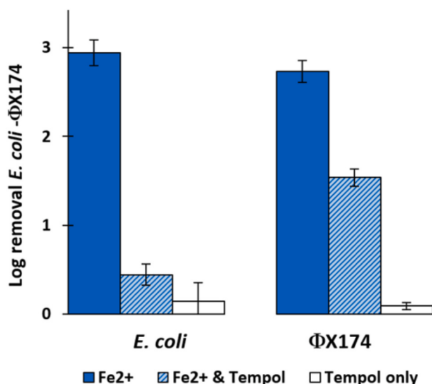
Fig. 5. Log Removal of E. coli WR1 (left) and somatic coliphage \Phi\text{X174} (right) under \text{Fe}^{2+} , \text{Fe}^{2+} + TEMPOL, and only TEMPOL (equimolar concentrations of 0.9 mM \approx 50 mgFe/l and/or 154.5 mgTEMPOL/l). Error bars represent standard deviation. All experiments were performed in duplicate and all microbial determinations were executed in triplicate.
