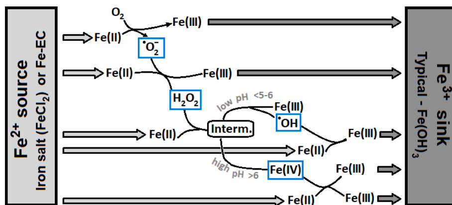
Fig. 1. Proposed pathways of aerobic \text{Fe}^{2+} oxidation, indicating the production of ROS: superoxide radical ( \text{O}_2^- ), hydrogen peroxide ( \text{H}_2\text{O}_2 ), hydroxyl radical ( \text{OH}^\bullet ) and high valent oxoiron ( \text{FeIV} ). Adapted from [15,18,39].
