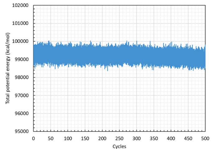
Fig. 19. Total potential energy in the aged bitumen during the fatigue simulations.
