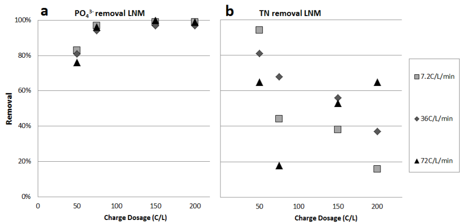
Figure 3-10 (a) \text{PO}_4^{3-} and (b) TN removal in Low Nutrient Medium (LNM) Fe-EC experiments
