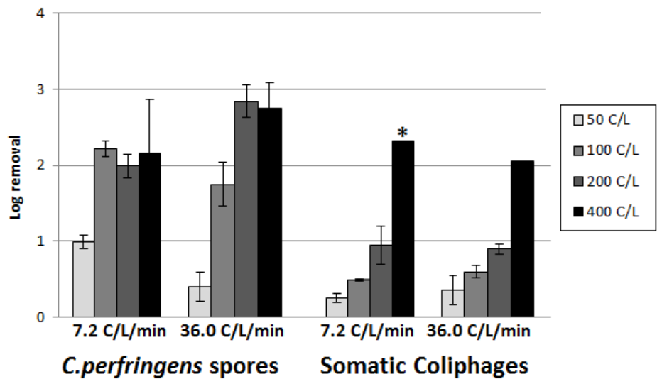
Figure 3-7 C. perfringens spores and somatic coliphage removal during real secondary effluent Fe-EC experiments. Note: Bars marked with an asterisk (*) indicate a minimum estimated removal due to effluent concentration below LOD. Each bar represents the average of two values (duplicate microbial screening, single assay). Error bars indicate standard deviation.
