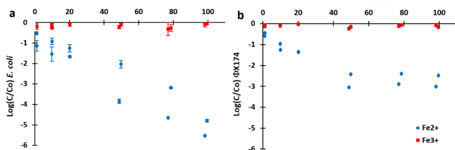
Figure 4-4 Inactivation of (a) E. coli WR1 and (b) somatic coliphage ØX174 during dosing 0-100 mg/l of either Fe 2+ or Fe 3+ . Error bars represent standard deviation. All experiments were performed in duplicate, and all microbial determinations were executed in triplicate.
