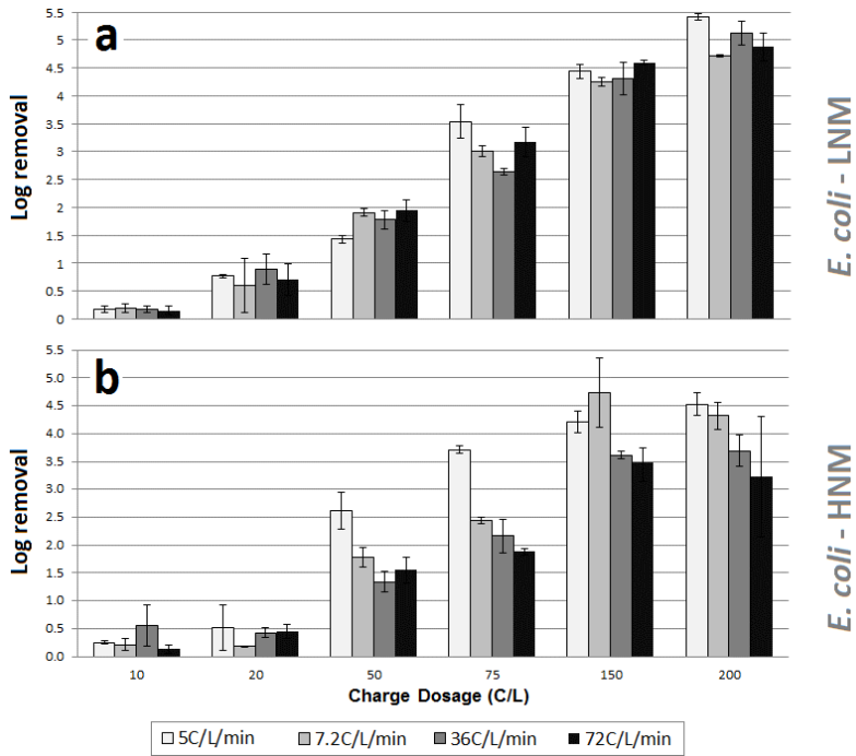
Figure 3-3 E. coli WR1 removal during Fe-EC experiments in LNM (a) and HNM (b) with increasing CD (10, 20, 50, 75, 150 and 200 C/l) and CDRs (5, 7.2, 36, 72 C/l/min). Each bar represents the average of four values (duplicate microbial screening in duplicate assays), error bars represent standard deviation.
