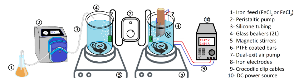
Figure 4-2 Fe dosage bench scale setup, with chemical dosage (left) and electrochemical dosage (right).
