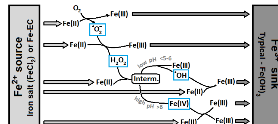
Figure 4-1 Proposed pathways of aerobic \text{Fe}^{2+} oxidation, indicating the production of ROS: superoxide radical ( \text{O}_2^{\cdot-} ), hydrogen peroxide ( \text{H}_2\text{O}_2 ), hydroxyl radical ( \text{OH}^{\cdot} ) and high valent oxoiron ( \text{FeIV} ). Adapted from Hug & Leupin, 2003, Kim et al., 2011 and Van Genuchten & Peña, 2017.
