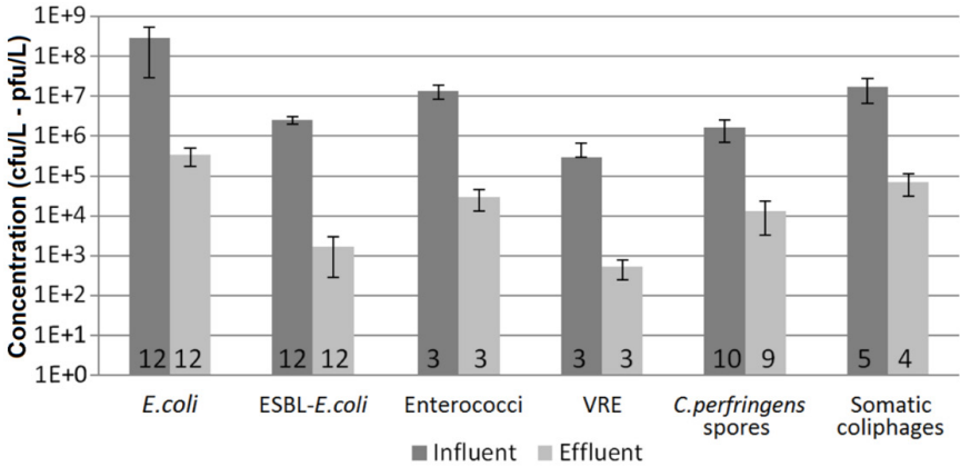
Figure 3-2 Microbial indicators E. coli , ESBL- E. coli , enterococci, VRE, C. perfringens spores and somatic coliphages in raw influent and secondary effluent of a conventional Dutch WWTP. Number of samples analysed for each indicator is noted on the foot of each bar. Error bars represent standard deviation.
