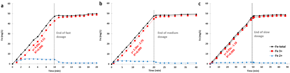
Figure 4-8 Fe profiles (Total Fe, Fe 2+ and Fe 3+ ) during (a) fast dosage (b) medium dosage and (c) slow dosage. The best fitting linear equation and R 2 for the Fe 3+ series (during Fe supply) is indicated in each case, together with the timestamp in which Fe supply is stopped. All experiments were performed in duplicate.
