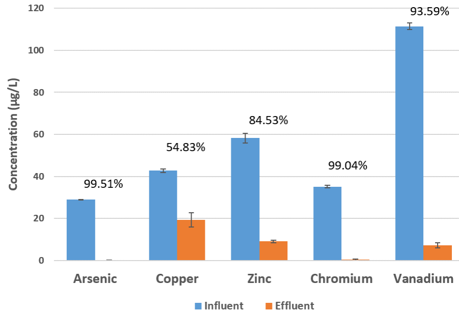
Figure 6-2 Preliminary data on heavy metal removal percentages using continuous flow Fe-EC on 2 nd effluents complemented with Arsenic (V), Copper, Zinc, Chromium and Vanadium. Experiments were performed in duplicate, and samples were analysed in triplicates. Error bars represent standard deviation.
