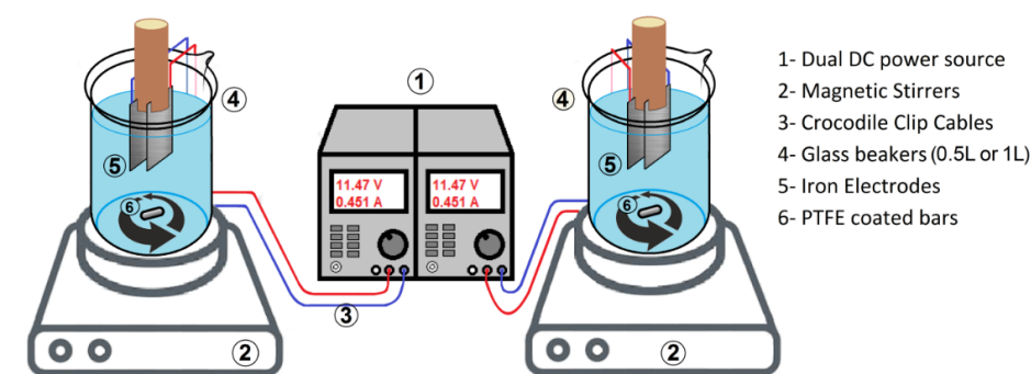
Figure 3-1 Bench scale EC laboratory setup
