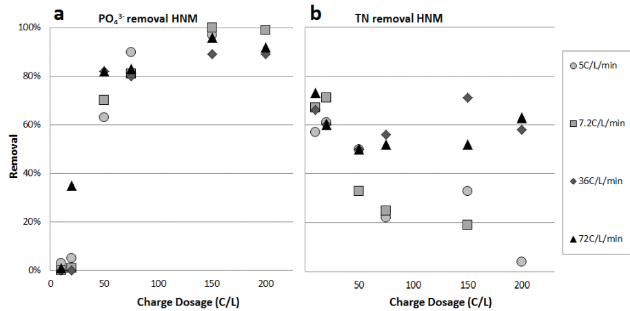
Figure 3-9 (a) \text{PO}_4^{3-} and (b) TN removal in High Nutrient Medium (HNM) Fe-EC experiments
