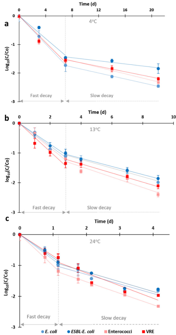
Figure 2-2 Log 10 data series of the relative microbial concentration (C/C 0 ) for E. coli , ESBL- E. coli , Enterococci and VRE on secondary municipal effluent stored at a) 4°C b) 13°C and c) 24°C. Experiments were performed in duplicate. Microbial screening was performed in quadruplicate for T=0, and triplicate for the rest of the samples. Error bars indicate standard deviation.
