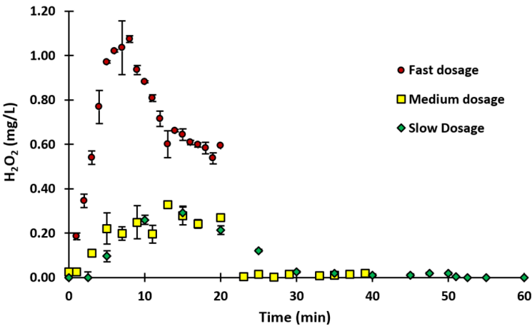
Figure 4-9 Average H 2 O 2 production profiles during fast, medium and slow Fe dosage. All experiments were performed twice. Error bars represent standard deviation.
