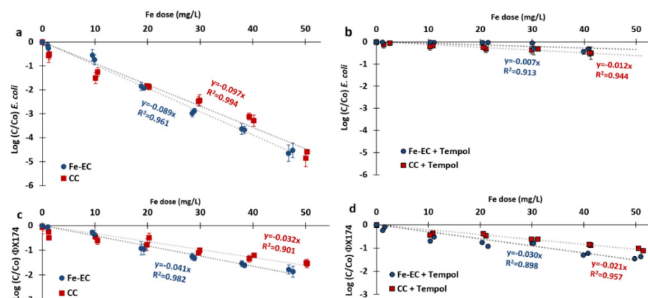
Figure 4-6 Inactivation of E. coli under CC and Fe-EC without TEMPOL (a) and with TEMPOL (b), and inactivation of phage ØX174 under CC and Fe-EC without TEMPOL (c) and with TEMPOL (d). Error bars represent standard deviation. All experiments were performed in duplicate, and all microbial determinations were executed in triplicate.
