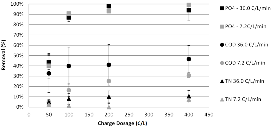
Figure 3-8 Removal of phosphate, COD and TN for real secondary effluent experiments. Each data point represents the average of four values (duplicate chemical screening in duplicate assays). Error bars indicate standard deviation.
