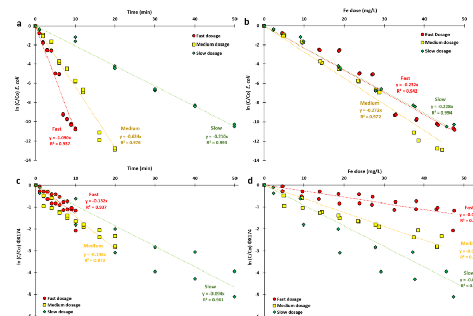
Figure 4-7 \ln(C/C_0) plot for E. coli WR1 concentration during the application of fast, medium and slow electrochemical Fe dosage as a function of (a) time and (b) dosed Fe, and \ln(C/C_0) plot for phage ØX174 concentration during the application of fast, medium and slow electrochemical Fe dosage as a function of (c) time and (d) dosed Fe. All experiments were performed in duplicate, and all microbial determinations were executed in triplicate.
