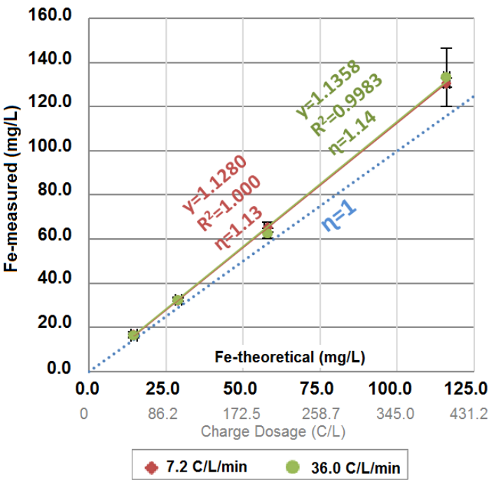
Figure 3-11 Faradaic efficiency calculation for real secondary effluent experiment (adjusted by least squares) of experiments under 7.2 C/l/min and 36.0 C/l/min. Error bars represent standard deviation ( n=4 ). Dotted line represents 100% Faradaic efficiency.
