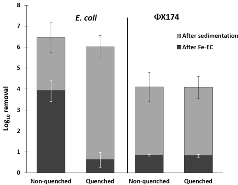
Figure 5-5 Log 10 removal plot of E. coli WR1 and phage ØX174 after Fe-EC, with and without the presence of the Fenton-inhibitor TEMPOL after Fe-EC and after 4h settling, indicating the independent contributions of ROS inactivation and floc sedimentation. Experiments were performed in duplicate, and microbial screening was performed in triplicate. Error bars indicate standard deviation.
