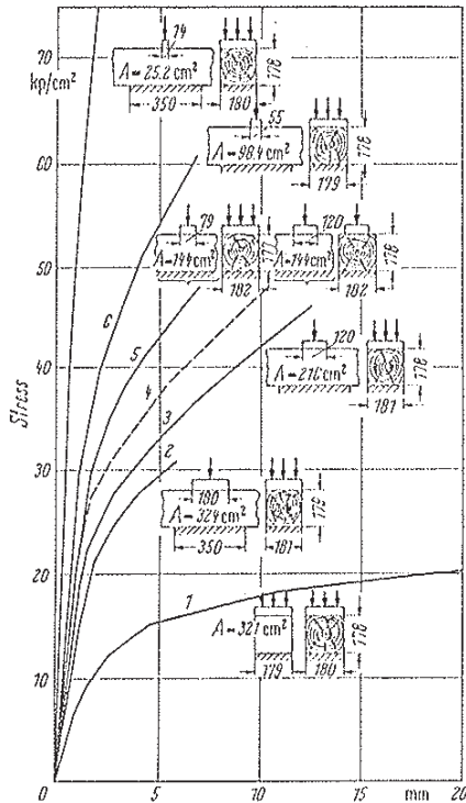
Local loading perp. to the grain [1] Graf Possible spreading
