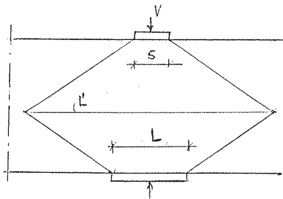
Local loading perp. to the grain [1] Graf Possible spreading
